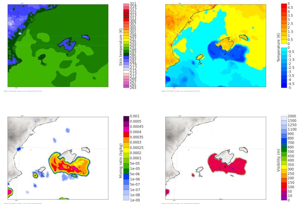
Figure 2. Modelled development of fog around the Balearic Islands, +030 h. ( Top row ): surface temperature (K), ( left ); difference between 2 m temperature and surface temperature (K), ( right ). ( Bottom row ): liquid–water mixing ratio (kg/kg), ( left ); visibility (m), ( right ).
