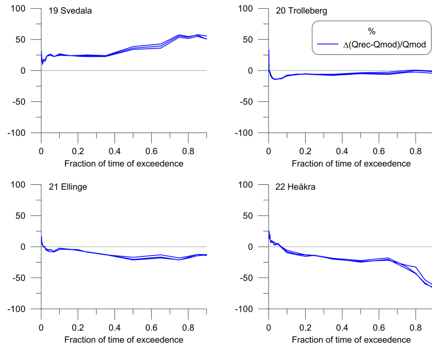
Figure 4. Impact of urbanization on discharge at different frequencies in the duration curve, modeled with S-HYPE (three model versions). The graphs show how the observed-modeled flow has changed from the period before 1991 to the period thereafter. A positive change is interpreted as an increase in discharge, and vice versa. Locations of catchments are given by corresponding numbers in Figure 1.
