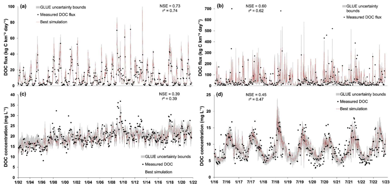
Fig. 3. Observed and simulated daily DOC flux and DOC concentrations for Vattholma (a and c) and Glenamong (b and d) catchments during model calibration. NSE and r^2 values are indicated for the calibrated parameter set (best optimised simulation). The grey area denotes the 5–95 % range GLUE uncertainty bounds for DOC flux and DOC concentrations based on the 100 best-performing parameter sets.
