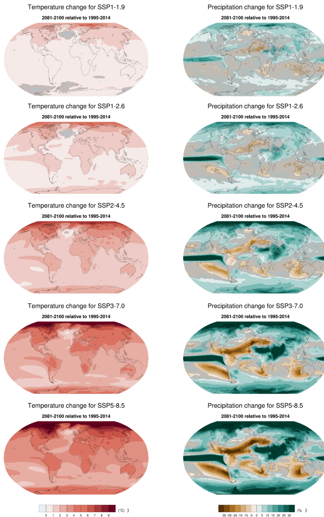
Figure A4. Patterns of changes by 2081–2100 relative to 1995–2014 in surface air temperature (°C) and precipitation (%) under the five scenarios. Stitched areas are not significant; i.e., the magnitude of the change does not exceed the models' standard deviation.
