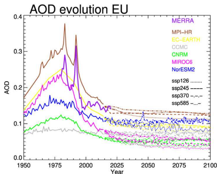
FIG. 3. AOD500 time series of GCMs selected as boundary conditions over Europe for different SSPs.
