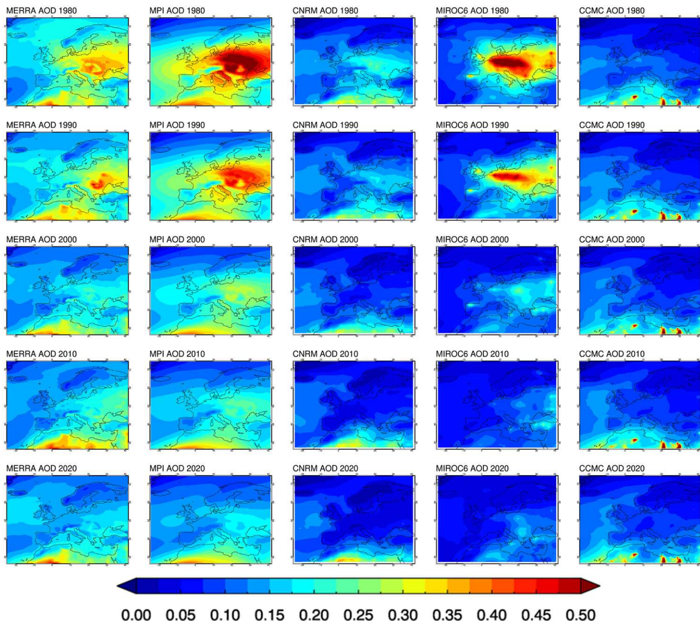
FIG. 2. Annual means for selected years of AOD550 over Europe for MERRA reanalysis and selected CMIP6 GCMs.
