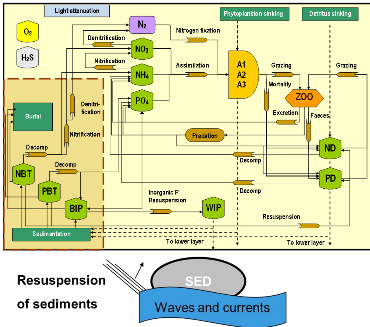
Figure 1. Schematic figure of the components of the SCOBI model as presented in Almroth-Rosell et al. (2015). The NEMO-Nordic-SCOBI model include in addition also the dynamics of Silicate (Kuznetsov et al., 2016), not shown in figure.
