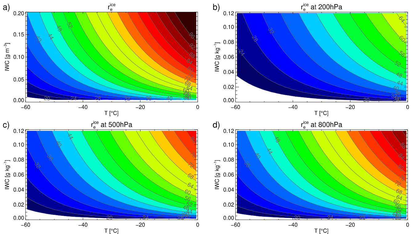
Figure 1. (a) Modeled ice effective radius ( r_e^{\text{ice}} ) in \mu\text{m} as function of temperature and cloud water content (given in \text{g m}^{-3} ) following Sun and Rikus (1999). (b) to (d) Modeled ice effective radius (in \mu\text{m} ) as function of temperature and cloud water content when given in \text{g kg}^{-1} at 200 hPa (b), 500 hPa (c) and 800 hPa (d). In atmospheric models the cloud water content is often given in \text{g kg}^{-1} , thus a small air pressure dependency is introduced into the calculation of the effective radius as the conversion from \text{g kg}^{-1} to \text{g m}^{-3} requires the air density which is a function of pressure.
