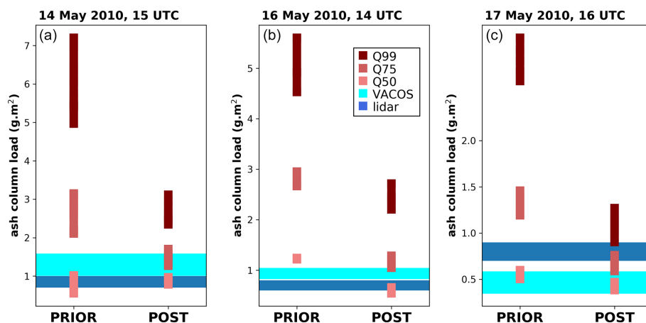
Figure 9. Comparison of ash load (vertical axis, unit \text{g m}^{-2} ), for the a priori (PRIOR) and a posteriori (POST) ensembles (abscissa), at the location of lidar measurements shown in Fig. 3, on 14 May at 15:00 UTC (a), on 16 May at 14:00 UTC (b), and on 17 May at 16:00 UTC (c). The range of lidar, or VACOS, estimates along the flight track are plotted as blue, or light blue, horizontal rectangles. Note that, in these cases, lidar and VACOS values do not overlap. The different quantiles ( Q50 , Q75 , Q99 ) are plotted as different red tones: the darker the colour, the higher the quantiles. For all data, the values of several grid points are plotted that sample the column loads along the flight track. Note the different y-axis scales.
