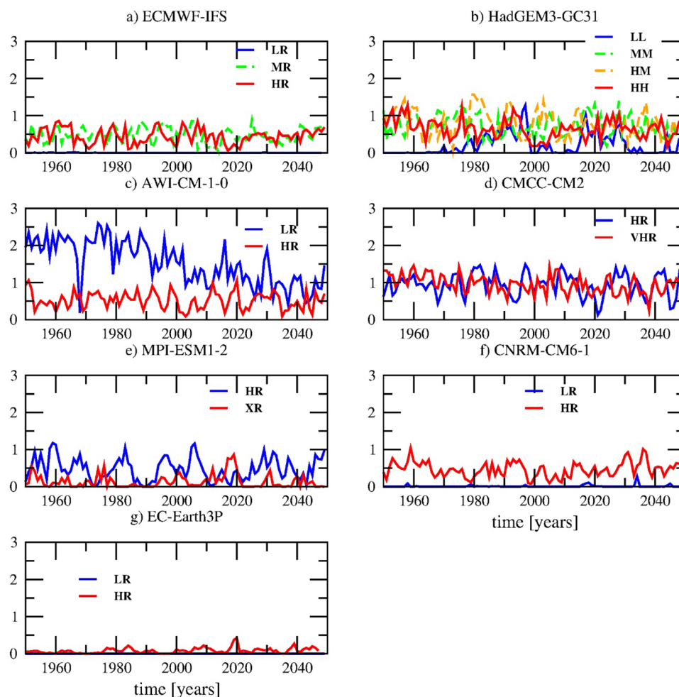
Fig. 4 As Fig. 3 but for the 100-year control simulation
