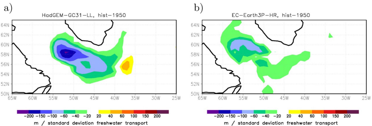
Fig. 11 Regression between annual mean freshwater transport through the Denmark Strait and mixed layer depth in the following March. a HadGEM-GC31-LL and b EC-Earth3P-HR. Data have been detrended before calculating the regression. These two simu-
