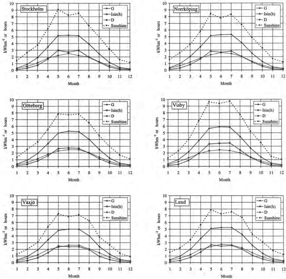
Figure 5.3. Mean daily sums 1983-1998 of global irradiation, direct horizontal irradiation ( I \sin(h) ), diffuse irradiation ( \text{kWhm}^{-2} per day) and duration of sunshine (hours per day) at the six southernmost Swedish solar radiation stations. Here the letter I instead of E_b is used for direct radiation.
