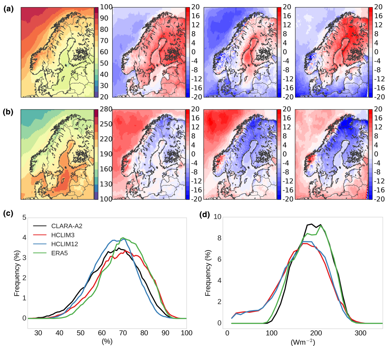
Fig. 8 Summer (JJA) mean of a : total cloud cover fraction (clt in percent) and b : shortwave down-welling radiation at the surface (SWd in \text{W/m}^2 ), in CLARA-A2 and percentage differences in HCLIM3,
