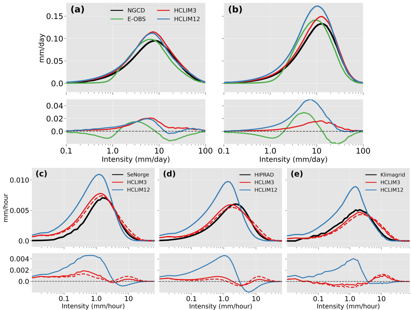
Fig. 9 Actual contributions per intensity bin to the total mean precipitation, units in mm per time unit. DJF (a) and JJA (b) daily precipitation over Fenno-Scandinavia, and, JJA hourly precipitation over Norway (c), Sweden (d) and Denmark (e) compared to national high-resolution data sets (see Table 1). Lower panels in each row show the differences compared to reference observations (given by
