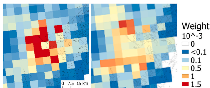
Fig. 13. Normalized PM 2.5 emission distribution in Stockholm from the Nordic inventory on the left and the TNO-newRWC on the right.
