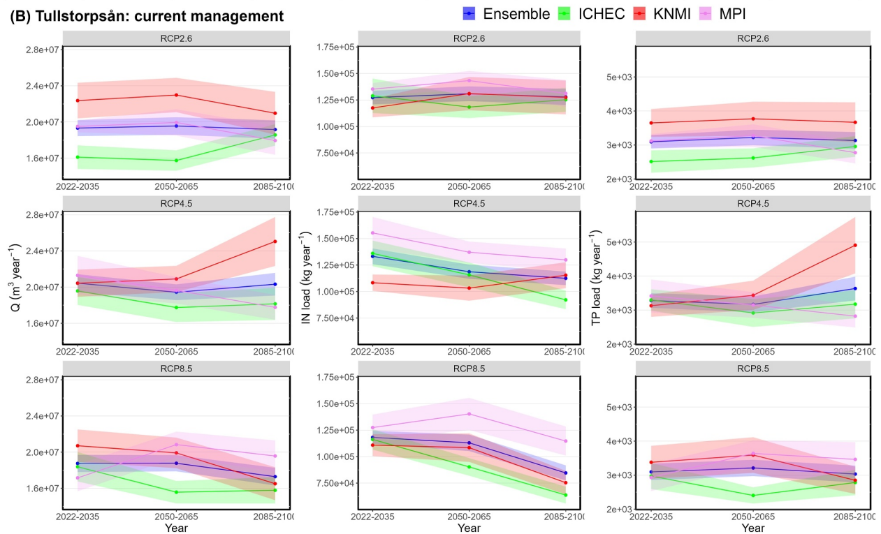
Figure 3. Changes in discharge and nutrient loads for the (a) Hestadbäcken and (b) Tullstorpsån catchments under different climate models and Representative Concentration Pathways. Results are for baseline management practices only. Point and lines represent the mean yearly loads for the period, while the ribbons represent one standard deviation.
