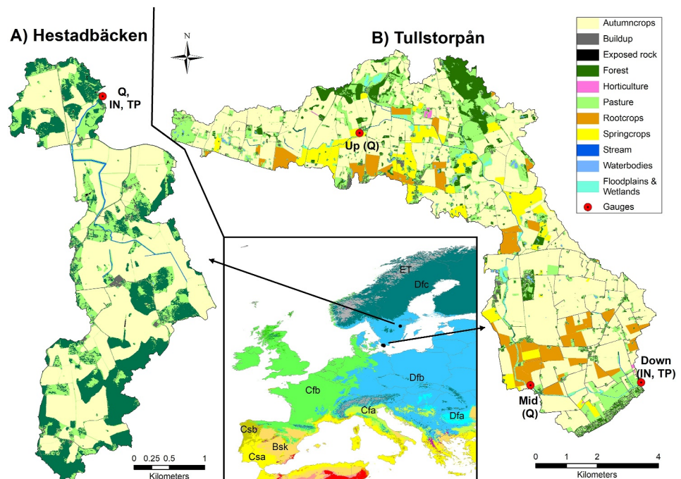
Figure 1. Location and climatic context of the study catchments within Europe under baseline conditions (Beck et al., 2018). Detailed land cover maps of (a) Hestadbäcken and (b) Tullstorpsån catchments, with location of the stream gauges used for calibration and validation.
