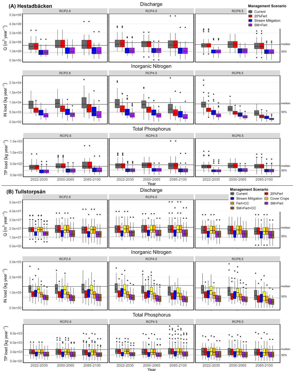
Figure 4. Effects of management scenarios on discharge, IN and total phosphorus loads under different Representative Concentration Pathways. The boxplots depict the outcomes from the ensemble climate model, where median values are shown by the central line, interquartile range by boxes, the range by whiskers, and the outliers by points. The black and dotted lines on the plots show the respective median value and 50% reduction to the baseline management scenario in the 2022–2035 period.
