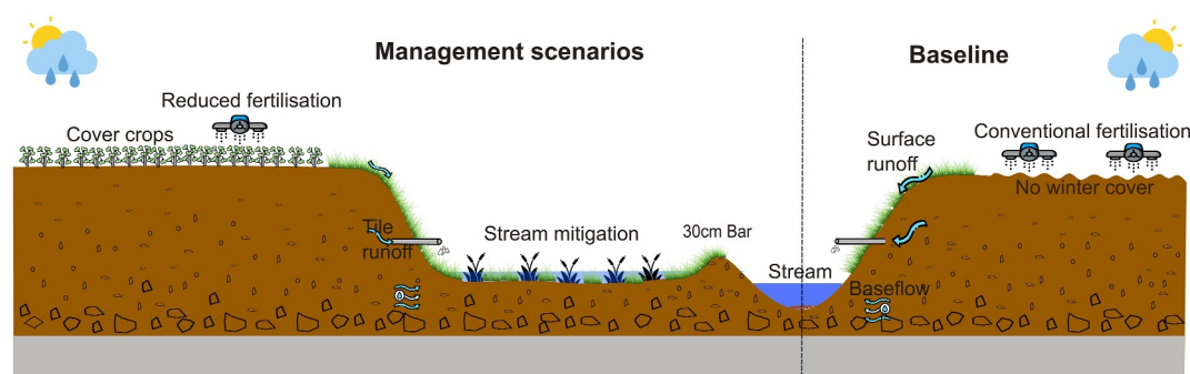
Figure 2. Schematic representation of the flow pathways and modeled management scenarios compared to the baseline.
