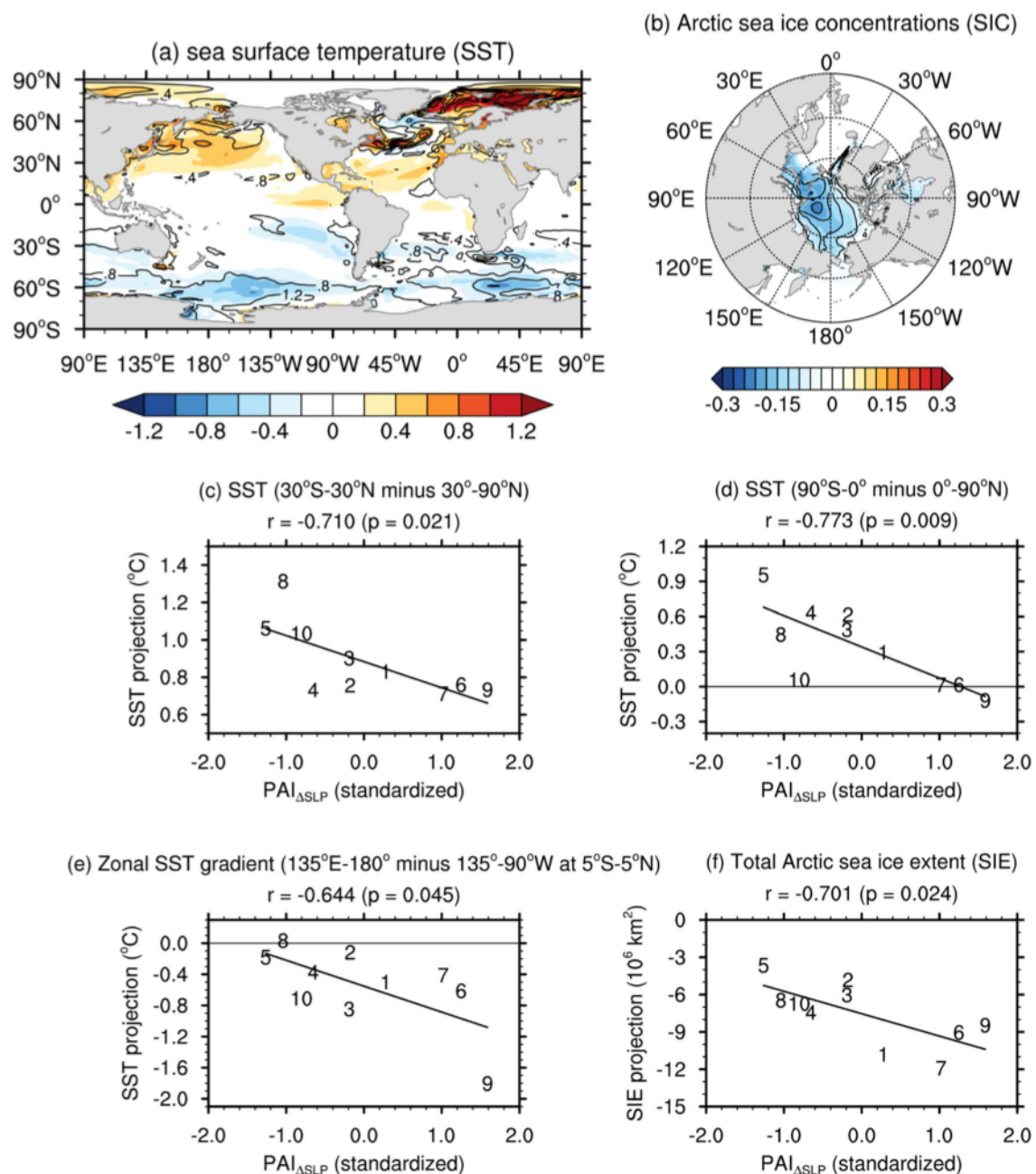
Fig. 4 a–b Inter-model regression of the forced response against PAI_{\Delta SLP} (shading) and the uncertainty in the forced response (i.e., inter-model standard deviation; contour) of the ten CMIP5 models: (a) SST (contour interval: 0.4 °C), (b) SIC (contour interval: 0.1 fraction), where the outermost circle in the polar stereographic map
