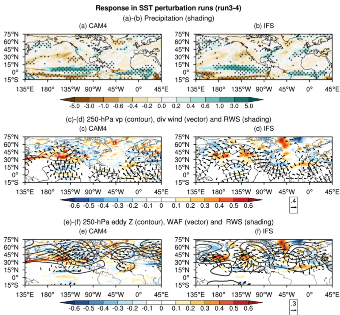
Fig. 12 As in Fig. 7, but for the response in the SST perturbation runs: (left) CAM4 and (right) IFS
