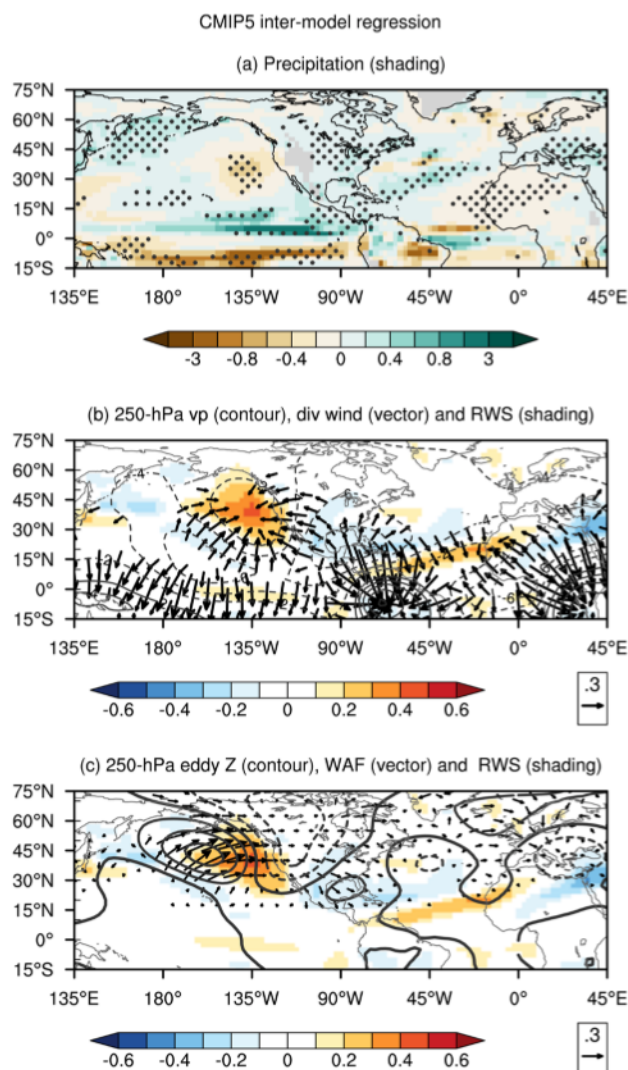
Fig. 7 Inter-model regression of the forced response against PAI_{\Delta SLP} across the ten CMIP5 models. a Precipitation (shading; mm\ day^{-1} ). b 250-hPa velocity potential (contour; 10^5\ m^2\ s^{-1} ), divergent wind (vector; m\ s^{-1} ), and Rossby wave source (shading; 10^{-11}\ s^{-2} ). c 250-hPa eddy geopotential height (contour interval: 10 m) and horizontal component of wave activity fluxes (vector; m^2\ s^{-2} ), and Rossby wave source (shading; 10^{-11}\ s^{-2} ). Stippling in (a) indicates the 95% confidence level
