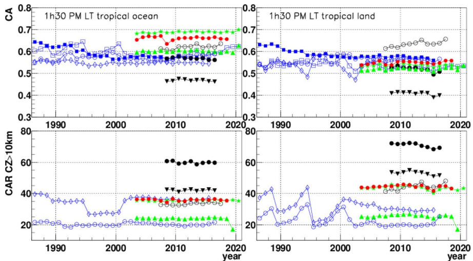
Fig. 12 Time series of cloud amount (top) and relative proportion of clouds with CZ > 10 km (bottom), over tropical ocean (left) and tropical land (right). Statistics at 1:30PM LT over 25N-25S. The colours correspond to specific instrument types (black: active LiDAR, red: IR sounders, green: advanced multi-spectral imagers, blue: multi-spectral imagers)
