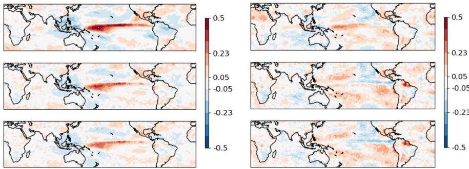
Fig. 14 Geographical maps of linear regression slopes between monthly mean anomalies in CAM_{col} (left) and CAL_{col} (right) and global mean surface temperature anomalies. Units are in fractional change per ^{\circ}C warming. The column amounts have been obtained from complementary information, as discussed in Sect. 4, using the CVL model for ISCCP (top), and using AIRS-CIRS combined with AVHRR-Cloud_cci (middle) or MODIS-CE (bottom). Surface temperature from the GISS Surface Temperature Analysis, during the period 2003–2015
