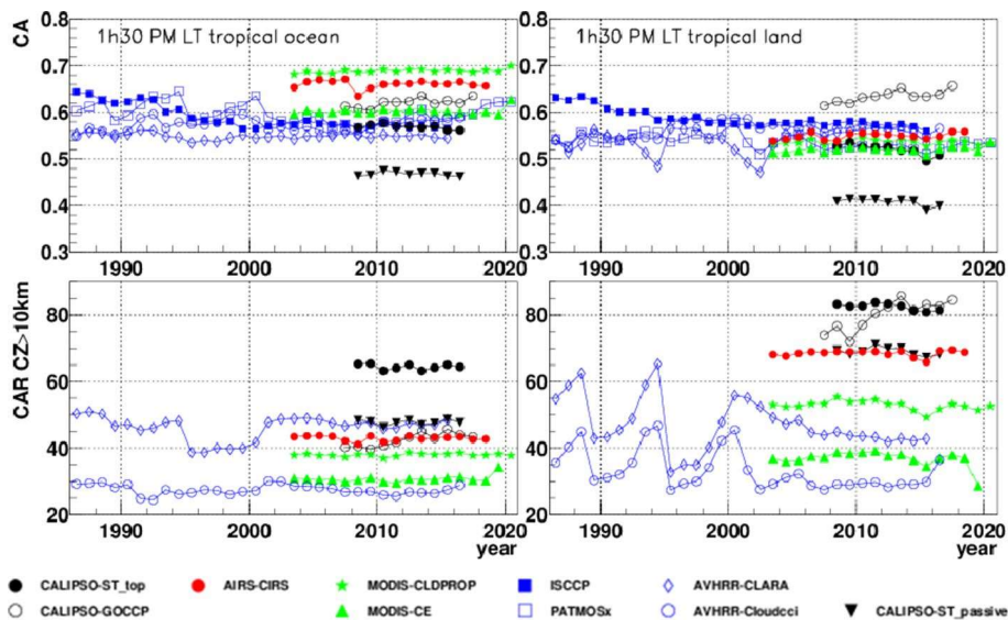
Fig. 12 Time series of cloud amount (top) and relative proportion of clouds with CZ > 10 km (bottom), over tropical ocean (left) and tropical land (right). Statistics at 1:30 PM LT over 25N–25S. The colours correspond to specific instrument types (black: active lidar, red: IR sounders, green: advanced multi-spectral imagers, blue: multi-spectral imagers)
