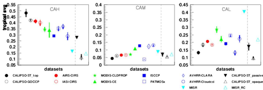
Fig. 3 Tropical (15N–15S) averages of height-stratified cloud amount (CAH, CAM and CAL) of the eleven datasets. CAH and CAM of clouds with COD>0.3 and of clouds with COD>3 from CALIPSO-ST as well as results from MISR_RC are also shown for comparison. Statistics averaged over day and night (1:30AMPM LT, except IASI (9:30AMPM) and MISR (10:30 AM)) over the common period of 2008—2015. The colours correspond to specific instrument types (black: active lidar, red: IR sounders, green: advanced multi-spectral imagers, blue: multi-spectral imagers, cyan: solar-spectral imager). The vertical bars indicate day (thick) and night (thin) differences with respect to the daily mean
