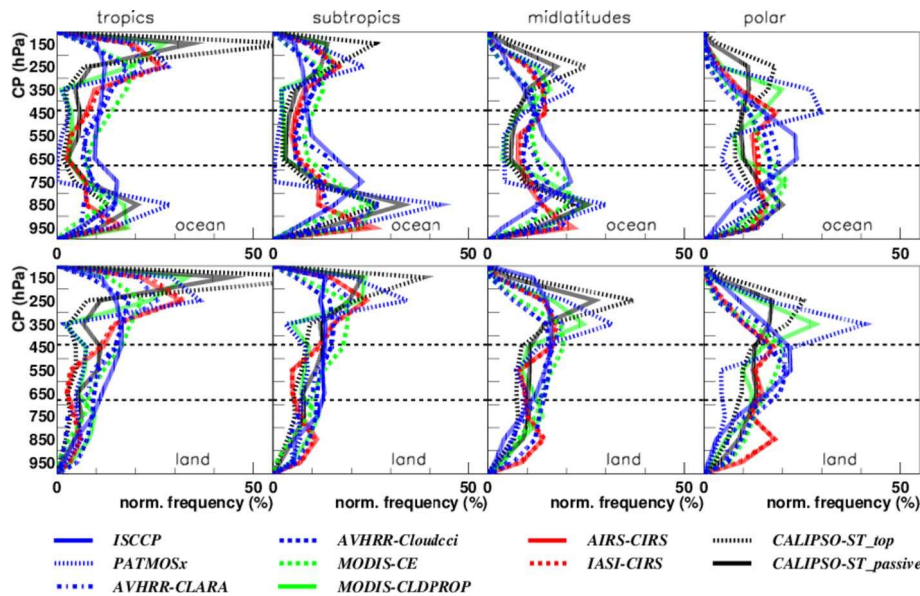
Fig. 6 Normalized frequency distributions of near-cloud-top pressure, CP, in four latitude bands (tropics: 10° N–10° S; subtropics: 10°–30°, mid-latitudes: 30°–60°; and polar: 60°–90°), separately over ocean (top) and over land (bottom). The frequency is given per 100 hPa. Statistics averaged over 1:30AM and PM LT (9:30AM and PM IASI). These normalized distributions only reflect a view from above, not considering hidden cloud layers. The colours correspond to specific instrument types (black: active lidar, red: IR sounders, green: advanced multi-spectral imagers, blue: multi-spectral imagers)
