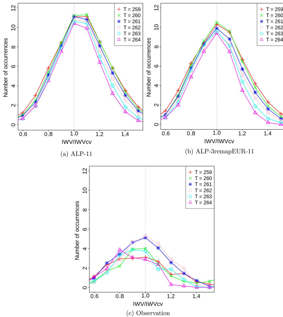
Fig. 11 Number of occurrence (units) of IWV rescaled by the corresponding onset threshold values IWVcv for precipitating days between ALP-11 (a), ALP3remapEUR11 (b) and observation (c) over the FPSCONV domain
