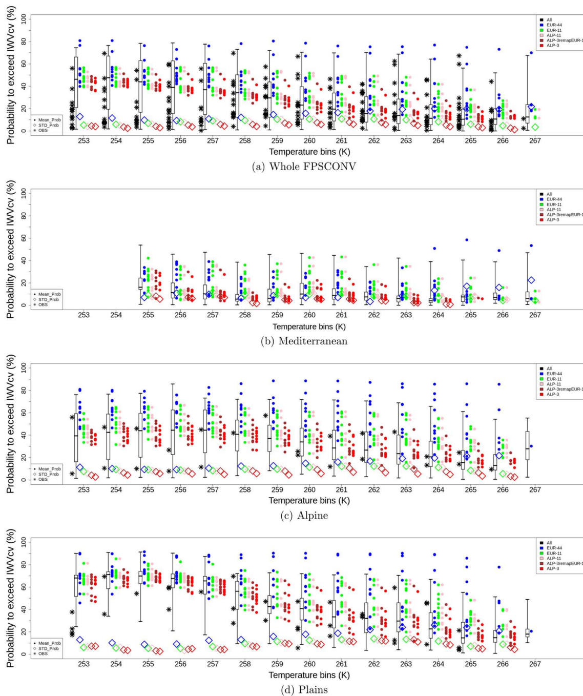
Fig. 7 Same as Fig. 6 but for probability to exceed IWVcv (%), the diamonds only show the standard deviation for each ensemble and have not been multiplied by 10
