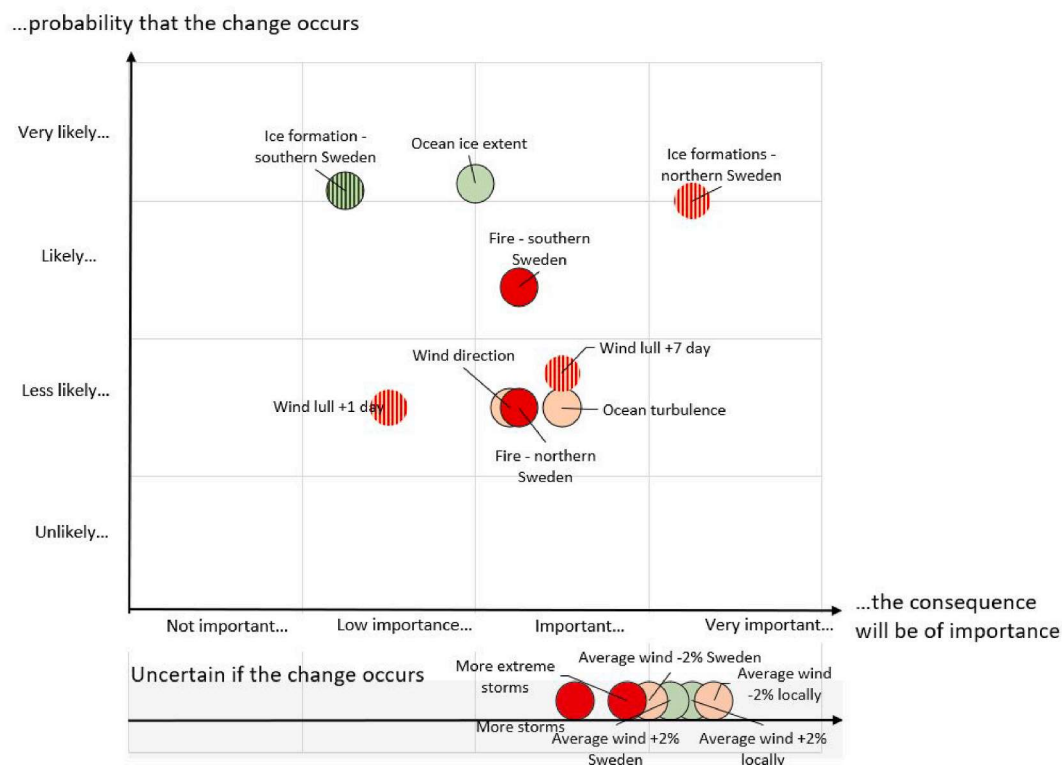
Fig. 6. Scatter plot for the wind power sector. Green colours: the consequence represents an opportunity for the sector. Red/orange colours: the consequence will lead to negative impacts. Light colours: the consequence impacts long-term operations and conditions. Dark colours: the consequence has short-term impact on operations. Vertical stripes: the consequence affects operations both in the long-term and short-term. Consequences for which the impact of climate change is uncertain are placed on a separate x-axis. Showing that the consequences are important and should be monitored further. (For interpretation of the references to colour in this figure legend, the reader is referred to the web version of this article.)
