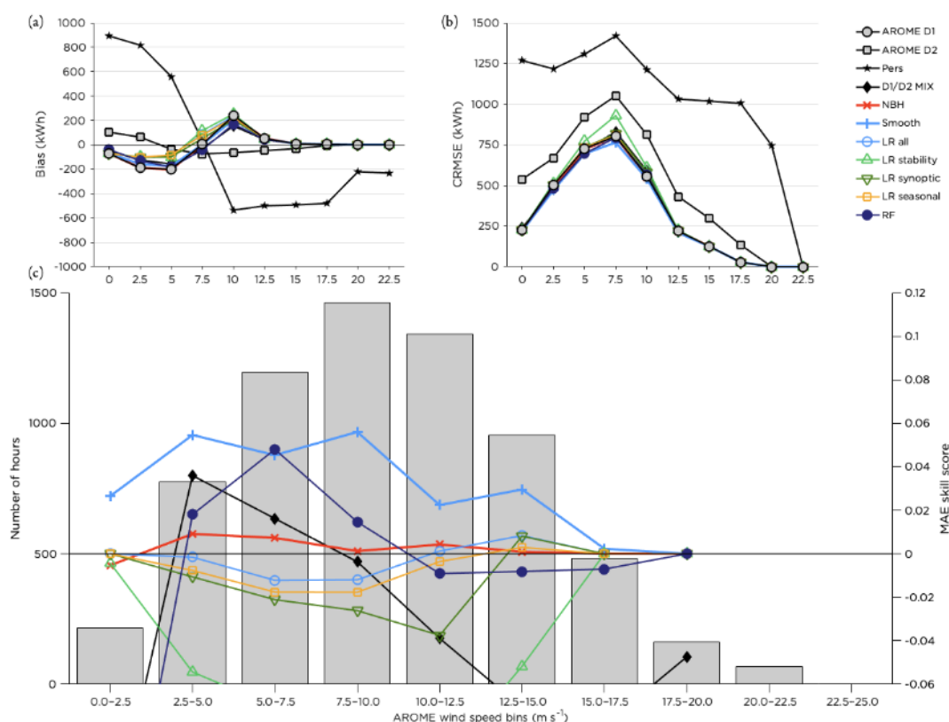
Figure 9. Performance of the post-processing methods for different wind speed bins. Panel (a) shows the bias, panel (b) the CRMSE and panel (c) the MAE skill score for the methods with the highest scores together with the distribution of the number of hours forecasted within each bin during the test period.
