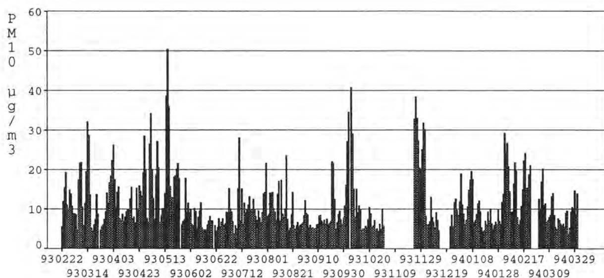
Figure 3.3 a. 24 hour averages of PM-10 at Aspvreten from 1993-02-22 to 1994-03-31 (all existing data at this site during the model test period).
