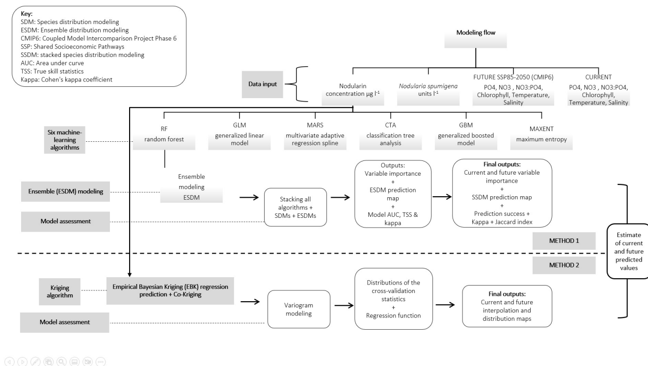
Figure 1. A diagram showing the modeling flow used to predict the present and future spatial occurrence of cyanobacteria and the toxin nodularin in the Baltic Sea.
