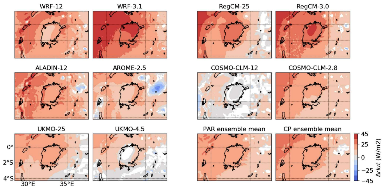
Fig. 12 Averaged upward longwave radiation at the top-of-the-atmosphere bias for all PARAmetrised (PAR) and Convection-Permitting (CP) models as well as the ensemble mean. The bias is calculated against the observational mean, while model values within the obser-
