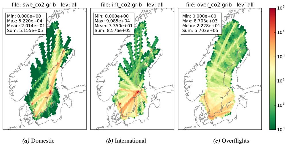
Figure 2: Total emissions for all altitudes (LTO, low cruise, high cruise) for CO 2 . Values are scaled according to table 3.
