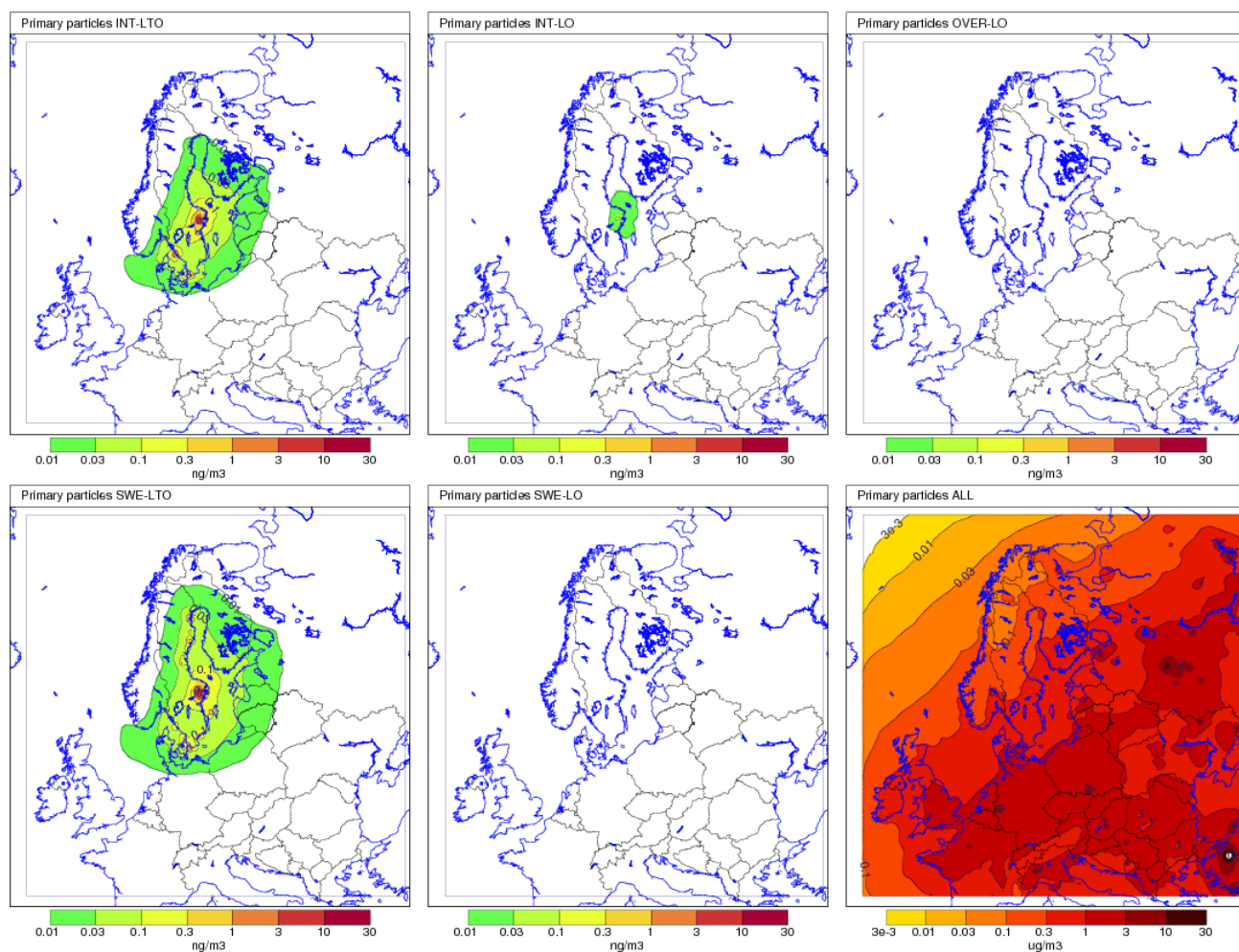
Figure 11: Yearly mean concentration of primary particles for year 2012-2014.
