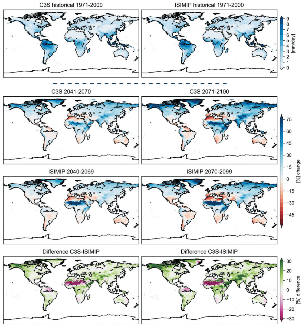
Figure 8. Historical mean annual precipitation (top row) and relative change in mean annual precipitation (bias-adjusted) for RCP8.5 for mid (2041–2070) and late century (2071–2100) with respect to the reference period (1971–2000): (second row) C3S ensemble mean; (third row) ISIMIP ensemble mean and (bottom row) difference between C3S ensemble mean and ISIMIP ensemble mean.
