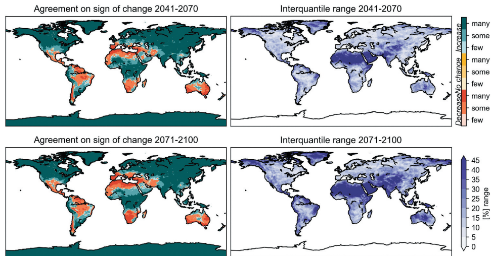
Figure 9. Confidence metrics for change in mean annual precipitation of the C3S data at the 0.5° resolution: agreement on sign of change (left) and inter-quantile range (right) for mid-century (2041–2070) and end of century (2071–2100).
