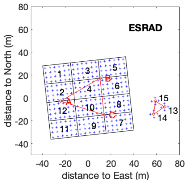
Figure 1. Configuration of the ESRAD antenna field. Each blue cross marks the position of a Yagi antenna in the main array (groups 1–12) and in the “remote” groups (13–15). Each group, 1–15, is connected to a separate receiver. Groups 1–12 are also connected to transmitters.
