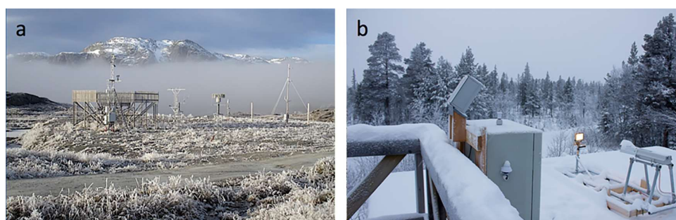
Fig. 1. (a) The MET-Norway Haukeliseter test site, which sits above tree line in the mountains of Telemark. (b) The IRF site in Kiruna, which is located in a boreal forest above the Arctic Circle in northern Sweden.
