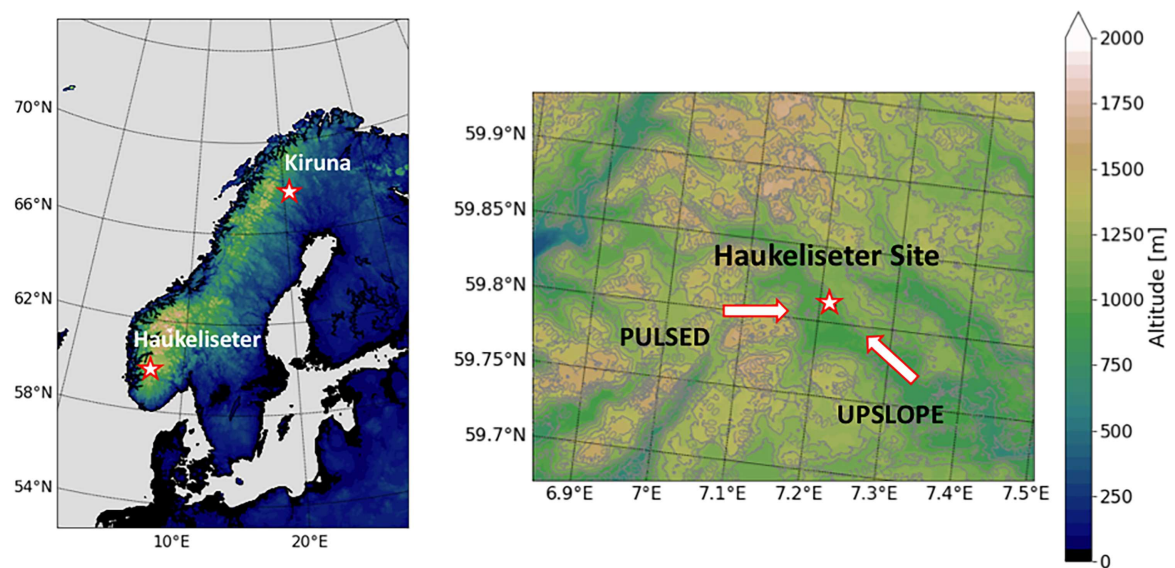
Fig. 2. (a) Location of HiLaMS field sites at Haukelisetter, Norway, in winter 2016/17 and Kiruna, Sweden, in winter 2017/18. (b) Topography and surface wind direction for two snowfall regimes observed at the Haukelisetter test site. Figure from S19.
