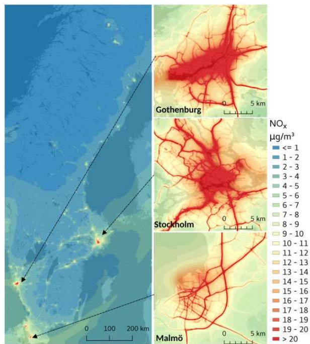
Figure 1 Average concentration of nitrogen oxides (year 2015) over Sweden (left panel) and the three largest cities in Sweden: Stockholm, Gothenburg, and Malmö (right panel). NO x = nitrogen oxides
