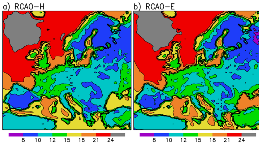
Figure 14. The average annual maximum 10 m wind speed ( \text{m s}^{-1} ) in the RCAO-H and RCAO-E control simulations.
