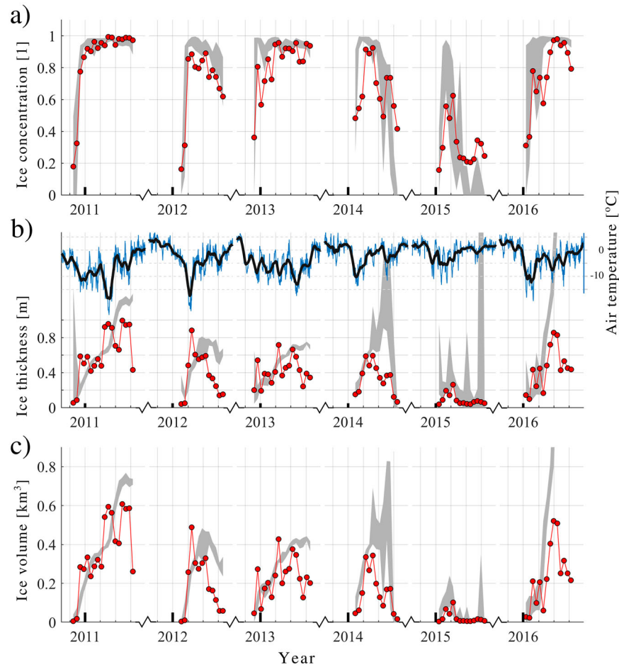
Figure 3.7.3. Time series of ice concentration (a), ice thickness (b) and ice volume (c) in the Bothnia Bay. Red dots show the CS2SMOS values. Shaded area represents the range of model values over the week centred at the CS2SMOS data derived time instant. Data from product references 3.7.1 and 3.7.2. Local (65.05°N, 23.23°E) air temperature time series are plotted on panel (b) (product reference 3.7.4). Blue line corresponds to 3-hourly data, thick black line corresponds to temperature time series smoothed using 30-day moving average filter.
