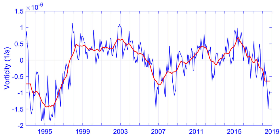
Figure 4.5.2. Time series of the spatially averaged current vorticity (blue line) and low-pass filtered (13 months) current vorticity (red line) computed in the Northern Ionian Sea (37–39°N; 17–19.5°E), during the period January 1993–November 2018. The temporal phases of the Northern Ionian Gyre are defined cyclonic when the vorticity field is positive and anticyclonic when the vorticity field is negative. Reference number of the product used: 4.5.1.
