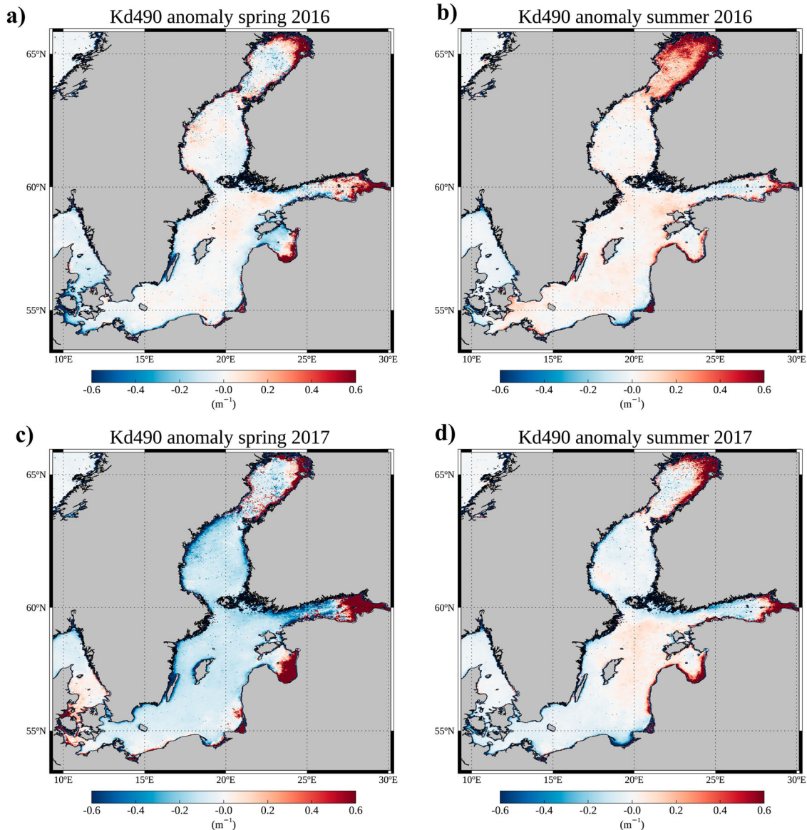
Figure 2.4.4. Attenuation coefficient ( K_d ) anomaly fields in spring 2016 (a) and 2017 (c) relative to the 1998–2014 spring mean field, and in summer 2016 (b) and 2017 (d) relative to the 1998–2014 summer mean field in the Baltic Sea. Data from product reference 2.4.1.
