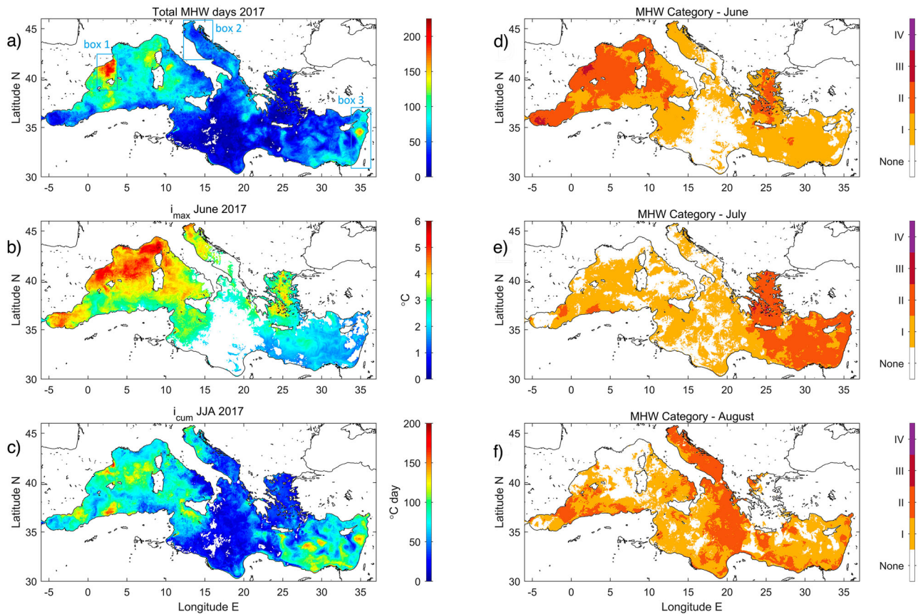
Figure 4.4.2. Maps showing different MHW metrics (left) and categorisation of MHW events by month (right). (a) Annual number of Marine Heat wave days in 2017, (b) MHW maximum intensity ( i_{\max} ) during June 2017, (c) June to August 2017 MHW cumulative intensity ( i_{\text{cum}} ). (d, e, f) Highest MHW category by month, during the regional MHW events of June, July and August. Locations with no heatwave days are blanked out. Reference number of the product used: 4.4.1. Location of the three boxes considered for sub-regional analysis and of the Scandola Marine protected Area are shown in panel a.
