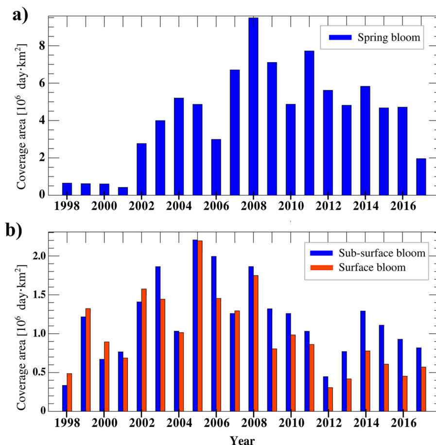
Figure 2.4.2. Time series of spring (a) and summer bloom (b) spatiotemporal coverage (day km 2 ) (1998–2017) using method by Hansson and Håkansson (2007). Results are based on CMEMS product reference 2.4.2 and 2.4.1 respectively.
