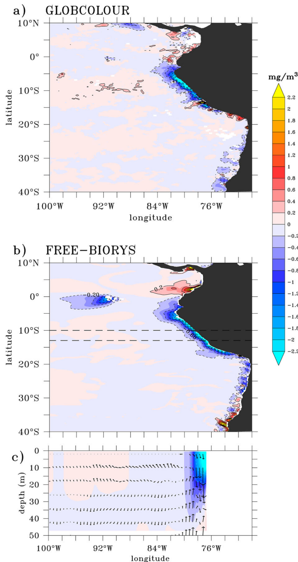
Figure 4.7.3. (a, b) Surface chlorophyll concentration anomalies (in mg/m 3 ), from the 2007–2017 climatology, for the month of March 2017 from (a) GLOBCOLOUR, and (b) the FREE-BIORYS product (products reference 4.7.3, 4.7.4). (c) Vertical section of chlorophyll concentration anomaly (shading) and current velocity anomaly (arrows), latitude-averaged over 10°S–13°S (dashed lines in b) in the upper 50 m. Anomalies are calculated from the climatological cycle. The current velocity has been vertically interpolated every 8 m.
