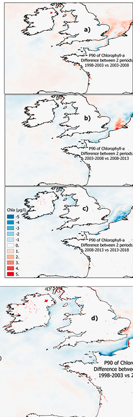
Figure 3.8.3. Differences of P90 of chlorophyll-a calculated over the productive period (March to October) on four periods of six years (a) 1998–2003 vs. 2003–2008, (b) 2003–2008 vs. 2008–2013, (c) 2008–2013 vs. 2013–2018. (d) 1998–2003 vs. 2013–2018. The results confirm that the most impacted regions by the decrease are the English Channel, the Irish Sea and the North Sea.
