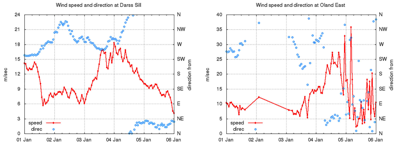
Figure 4.6.5. Hourly winds during the storm surge period at Darss Sill (54.7°N, 12.7°E, left) in the western Baltic Sea and Öland East station in the Öland East (56.92°N, 17.08°E, right). Note: the wind speed scale is different on the two graphs (product ref. 4.6.3).
