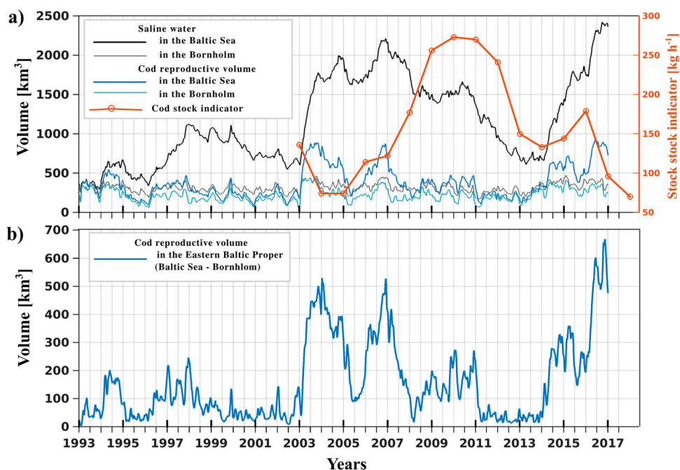
Figure 2.5.2. (a) Time series of saline water volumes (SWV, S > 11 \text{ g/kg} ) black line and cod reproductive volumes (CRV) in the Baltic Proper (thick lines), excluding Arkona Basin; and in Bornholm Basin (thin lines); and cod stock size indicator. Dots in the red line represent the geometric mean of the biomass of \geq 30 cod specimens in the previous year from the Baltic International Trawl Survey in subdivisions 25–28. (b) Time series of cod reproductive volume (CRV, S > 11 \text{ g/kg} , \text{O}_2 > 2 \text{ ml/l} ) extending outside the Bornholm Basin. Time series are calculated from CMEMS product reference 2.5.1 and 2.5.2.
