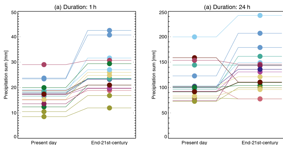
Figure 4. Modelled return levels at 50° N, 10° E (northern Germany; marked with a red cross in Fig. 1) for the present and future for a 10-year return period and 1 and 24 h durations. Different colours represent the 19 different GCM–RCM simulations listed in Table 1.
