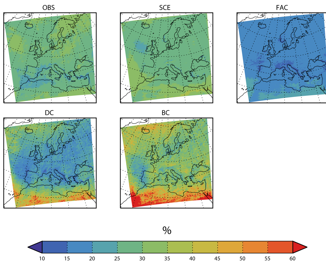
Figure 5. Geographical distribution of the relative error of the end-21st-century 10-year return level for a 1 h duration precipitation intensity from the inter-model cross-validation. Colours show the median of the relative error calculated over all model/pseudo-observation combinations. Panels show the different adjustment methods.
