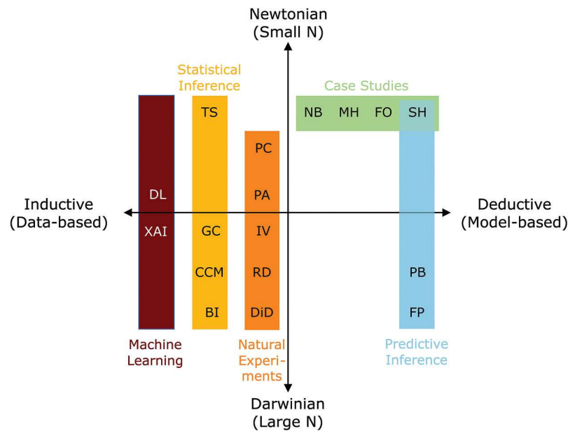
Figure 3. Approximative typology of attribution approaches: DL (diagnostic learning), XAI (explainable artificial intelligence), TS (time series analysis), GC (Granger causality analysis), CCM (convergent cross-mapping), BI (Bayesian inference), PC (paired catchments), PA (panel analysis), IV (instrumental variable), RD (regression discontinuity), DiD (difference-in-difference), NB (narrative-based analysis), MH (multiple hypotheses), FO (field observation), SH (socio-hydrological modelling), PB (process-based or physical modelling), FP (fingerprinting).
