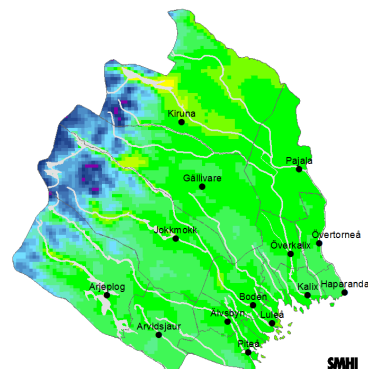
Observerat 1991-2013
