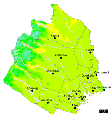
Observerat 1991-2013
