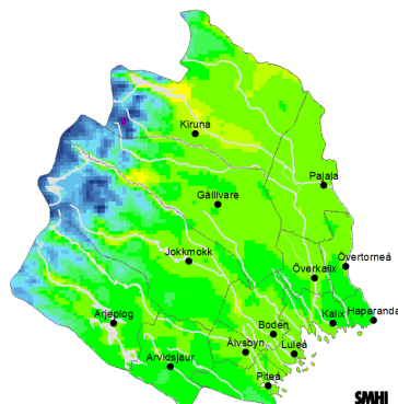
Observerat 1961-1990
