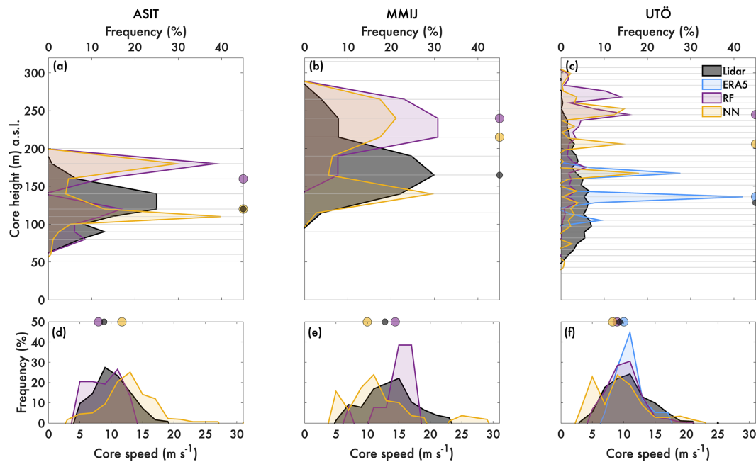
Figure 7. Distributions of LLJ core height (a–c) and core speed (d–f) for the three sites for the test period. For LLJ identification, crit. 1 is applied. The horizontal lines in panels (a–c) mark the height levels in the lidar measurements, i.e., the possible heights of LLJ cores. The circles mark the medians of each distribution, respectively. A threshold of at least 10 LLJs is set to plot the statistics, and thus, ERA5 data are missing for ASIT and MMIJ.
