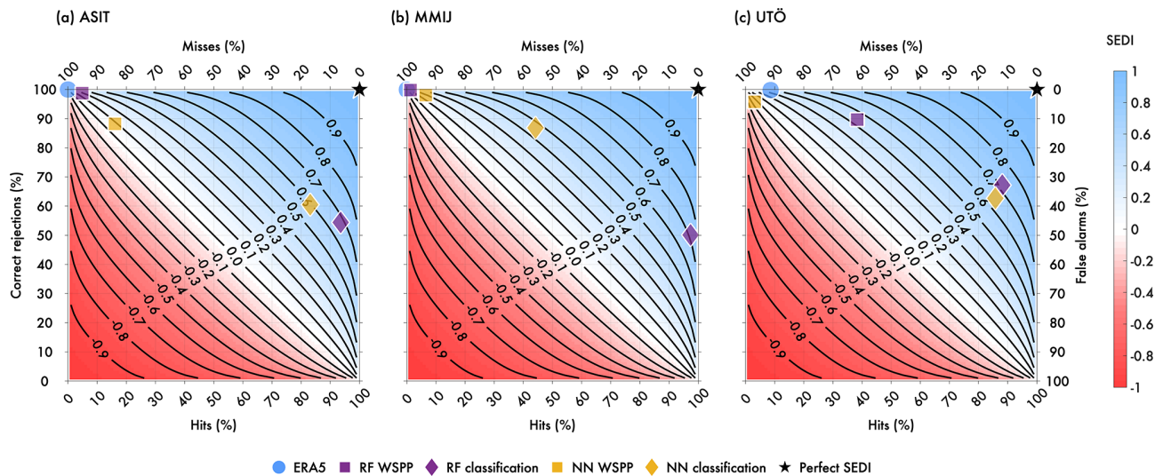
Figure 9. SEDI plots for (a) ASIT, (b) MMIJ, and (c) Utö. On the lower abscissa, the percentage of hits is plotted, i.e., the hit rate, and on the upper abscissa the percentage of misses. On the left ordinate the percentage of correct rejections is plotted and on the right ordinate the percentage of false alarms, i.e., the false alarm rate. The background coloring indicates the SEDI, which is also shown by the isolines. What would be a perfect SEDI (100 % hits, 0 % false alarms) is marked by the black pentagon in the top right corner of each panel. Results for the test period and SEDI for ERA5 (blue circles), RF (purple symbols), and NN (yellow symbols) are plotted.
