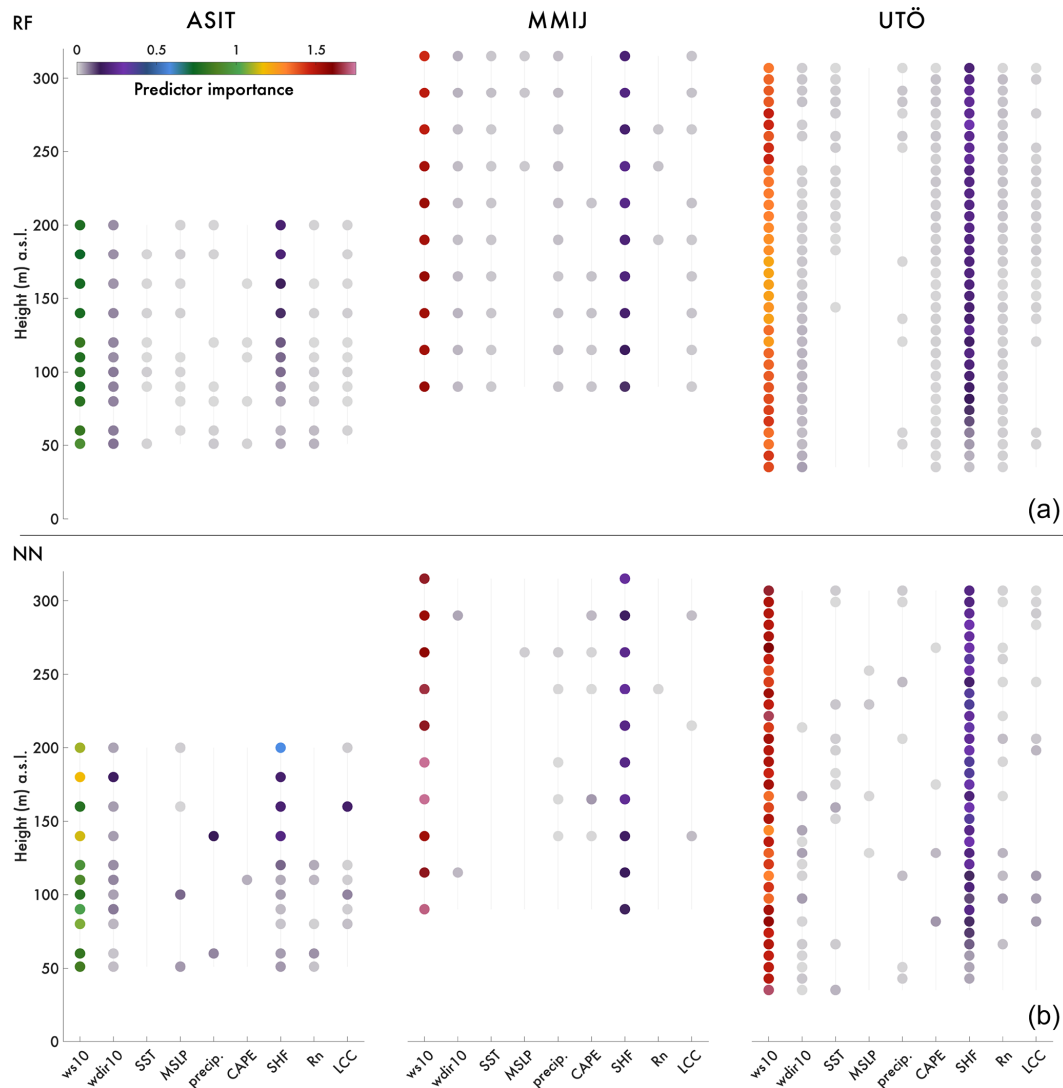
Figure 5. Predictor importance by height of each variable selected by the ML methods to predict the wind speed in the profile for each of the three sites and the two ML methods: (a) RF and (b) NN. The predictor importance denotes how important the predictor is to minimize RMSE between the model predictions and the ground truth lidar observations. ERA5 variables with highest predictor importance are indicated with colored circles. The predictor importance is calculated for the validation period.
