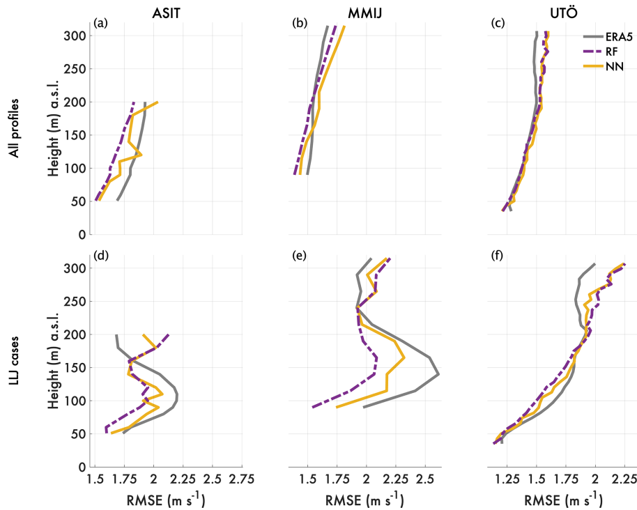
Figure 6. (a–c) RMSE for wind speed profiles for ERA5 (gray), the RF (purple), and the NN (yellow) for ASIT, MMIJ, and Utö. The values of RMSE are calculated relative to the lidar observations, and the results are valid for the test period. Panels (d–f) present RMSE for ERA5 and the ML models for the subset of the test data with LLJs (crit. 1) in the lidar profiles.
