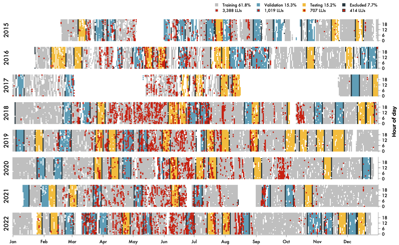
Figure 3. Overview of the data split for the Utö time series, February 2015–December 2022. The data were split into training (light gray), validation (blue), and testing (yellow) subsets and to minimize temporal auto-correlation one day of data before and after blocks of validation and testing are excluded (dark gray). Hours where there was an LLJ in the lidar profile are marked with red circles.
