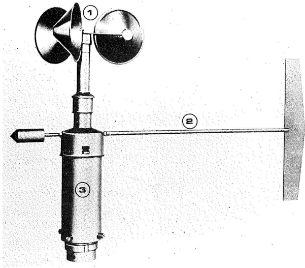
Figure 2. Söderlund cup anemometer used at SMHI observational station during the second half of the 20th century with cups (1), windvane (2), and transmission unit (3) (SMHI).
