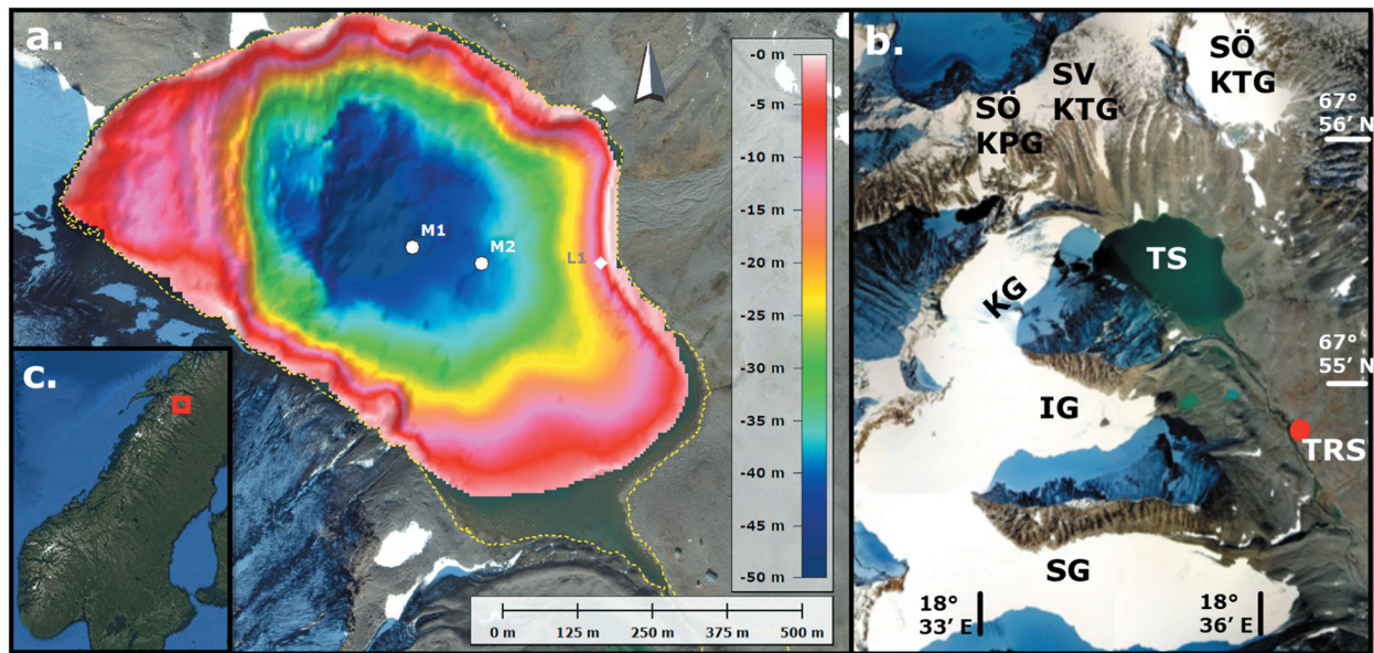
Figure 1. (a) Lake Tarfala, with color-coded high-resolution bathymetry from Kirchner et al. (2019) overlaid on orthophoto Rgb050 (GSD 2+ elevation data, Lantmäteriet 2015), showing also the terminus of Kebnepakteglaciären, formerly terminating in the north-western part of Lake Tarfala. Lake level (yellow stippled line) is at 1,162 m.a.s.l. White dots mark mooring sites M1 and M2. At M1, water temperature has been measured at various depths in the water column since 2016. The white diamond marks the site L1 where a StarOddi CTD sensor was moored. (b) The Tarfala area on a regional overview map from Google Earth (image: 10 August 2013) with Lake Tarfala (Tarfalasjön, abbreviated TS) in the center. Red dot marks the location of TRS. Storglaciären (SG), Isfallsglaciären (IG), and Kebnepakteglaciären (KG) are marked, as well as Sydöstra Kaskasapakteglaciären (SÖ KPG), Sydvästra Kaskasatjåkkaglaciären (SV KTG), and Sydöstra Kaskasatjåkkaglaciären (SÖ KTG). Note that Tarfala Bridge is located outside of the area shown in (b). (c) Location of the Tarfala area in northern Sweden (image from Google Earth).
