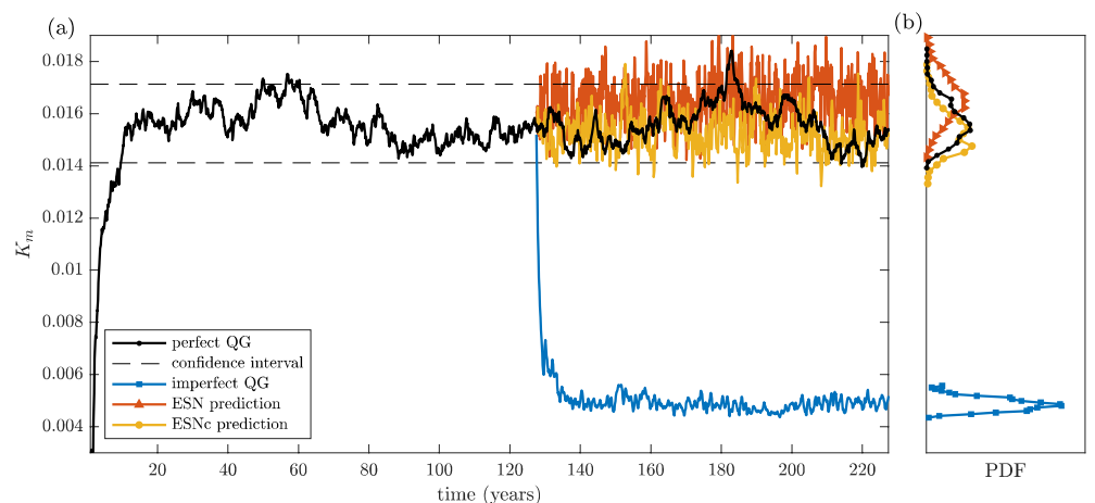
Figure 5. Spinup and long-term transient dynamics indicated by mean kinetic energy K_m . (a) A 100 years spinup with the perfect QG equations using a time step \Delta t = 1 day is followed by a training period of N_r \Delta t = T = 10,000 days. After the training period, 100 years predictions with imperfect QG, ESN and ESNc are shown, using N_r = 3,200 and \lambda = 1 . (b) Approximations of the probability density functions (PDFs) associated with the equilibrium transients, using 20 bins and excluding spinup/transition periods. Vorticity snapshots at the end of the depicted trajectories are shown in Figures 3 and 6. The ESN results are with single realizations and serve as a demonstration of the corrected dynamics.
