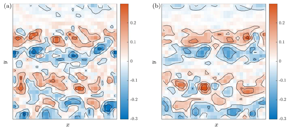
Figure 6. Snapshots of the vorticity fields (in \text{day}^{-1} ) at the end of the transient in Figure 5. (a) Standalone ESN prediction with N_r = 3,200 and \lambda = 1 , (b) hybrid ESNc prediction with N_r = 3,200 and \lambda = 1 .
