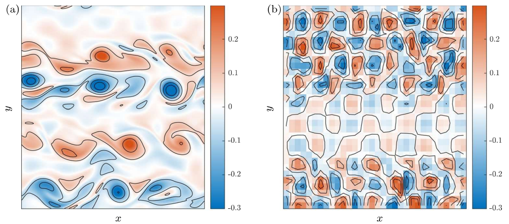
Figure 3. Snapshots of the vorticity fields (in \text{day}^{-1} ) at the end of the transient depicted in Figure 5. (a) Perfect model vorticity snapshot from a statistical equilibrium with N_f = 2 \cdot 256^2 and \text{Re}_f = 2,000 . (b) Imperfect model vorticity, also in a statistical equilibrium, N_c = 2 \cdot 32^2 and \text{Re}_c = 500 .
