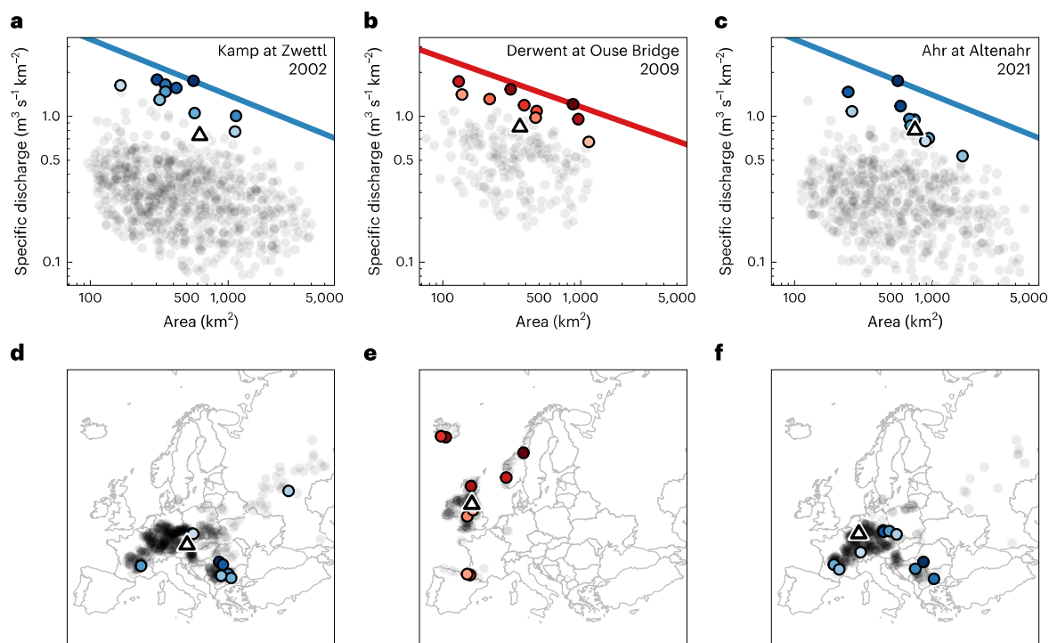
Fig. 2 | Envelope curves for three catchments with recent mega-floods in Europe. a–f, Kamp (622 \text{km}^2 catchment area) with 2002 flood (a,d), Cumbrian Derwent (363 \text{km}^2 ) with 2009 flood (b,e) and Ahr (746 \text{km}^2 ) with 2021 flood (c,f), indicated with triangles. Maximum specific discharges observed before the year of occurrence of the mega-flood for are shown for 824 (a), 196 (b) and 590 (c) similar donor catchments (points) selected within the corresponding hydroclimatic region. Coloured points indicate the ten largest events (in terms
