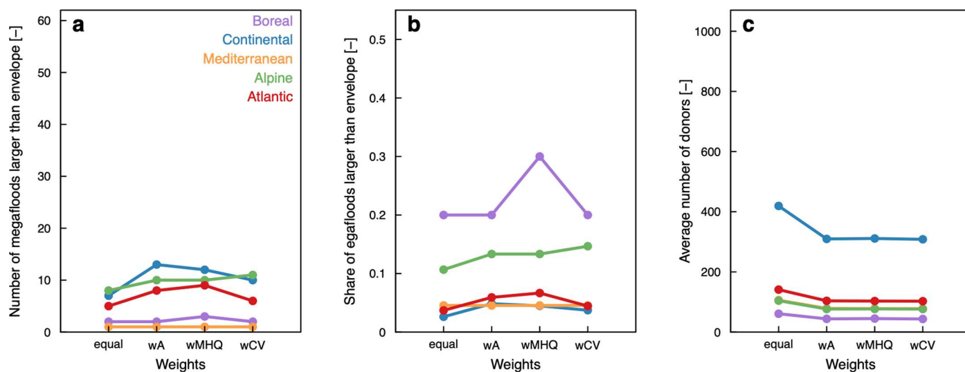
Extended Data Fig. 3 | Sensitivity of results to the weights used for estimating distance D. (a) Number and (b) fraction of megafoods larger than envelope for four weight combinations: equal weights ('equal', \alpha = \beta = \gamma = 1 ), double weight
