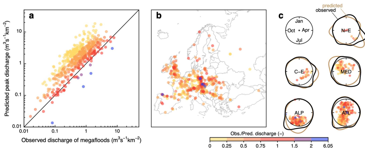
Extended Data Fig. 7 | Predicted versus observed megafloods. Similar to Fig. 4 but for the five alternative regions of Extended Data Fig. 4a. a , Predicted specific envelope discharge for 498 target catchments versus observed specific discharge of the megafloods in the same catchments. Predicted envelope discharges are estimated using discharge observations from a pool of donor catchments up to the year before the target megaflood. Colours indicate the ratio of observed and predicted discharge. b , Location of target catchments. Megafloods occur all over
