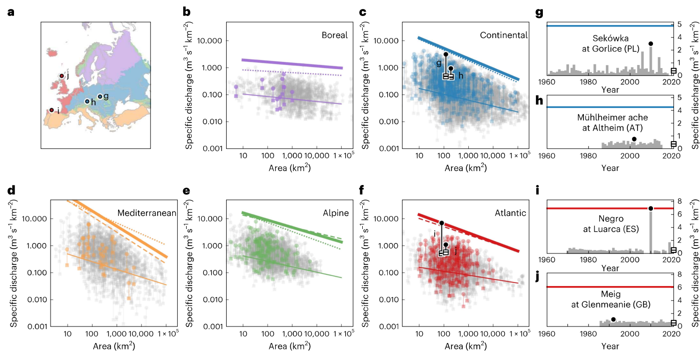
Fig. 1 | Megafloods in Europe. a , Five hydroclimatic regions: Boreal (purple), Continental (blue), Mediterranean (orange), Alpine (green) and Atlantic (red). b–f , Maximum observed specific flood discharges (points) and mean of annual specific flood discharges (squares) over the entire observation period at each stream gauge as a function of catchment area. Regional envelope curves (thick lines) and median regional annual specific flood discharges (thin lines) for the full record period are shown for each hydroclimatic region: Boreal ( b ), Continental ( c ), Mediterranean ( d ), Alpine ( e ) and Atlantic ( f ). Envelope curves for two 30-year sub-periods are also shown (dashed lines for 1961–1990, dotted lines
