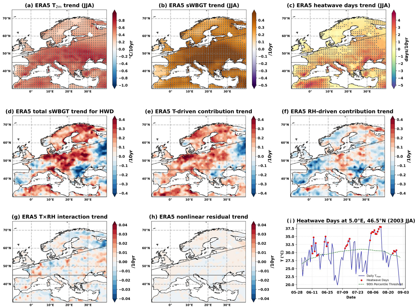
Figure 1. Trends in European summer heat stress and its drivers (1979–2023; ERA5). (a–c) Decadal trends in annual JJA mean 2m temperature ( T_{2m} ), annual JJA mean sWBGT, and annual number of heatwave days. (d–h) Trends during heatwave days (HWD) in total sWBGT and its temperature-driven, RH-driven, T \times RH interaction, and nonlinear residual contributions, respectively. (i) Schematic of the heatwave definition using summer 2003 data at 5.0°E, 46.5°N, showing daily maximum temperatures (blue line), the 90th percentile threshold (green dashed line), and heatwave days (red dots). Stippling indicates grid cells significant after adjustment for lag-1 temporal autocorrelation and Benjamini–Hochberg false discovery rate control at q = 0.05 .
