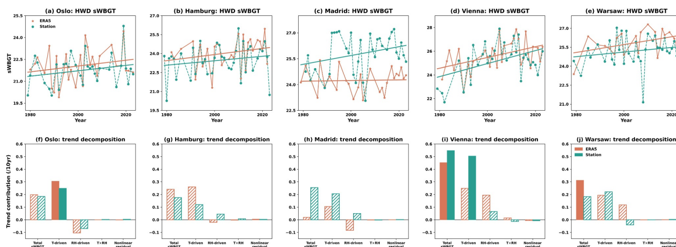
Figure 3. City-scale comparison of sWBGT during heatwave days, 1979–2023. (a–e) Annual sWBGT in Oslo, Hamburg, Madrid, Vienna, and Warsaw from ERA5 and station records. (f–j) Trends in total sWBGT and its temperature-driven, RH-driven, T \times RH interaction, and nonlinear residual contributions. Solid and hatched bars indicate p < 0.05 and p \geq 0.05 , respectively, after lag-1 autocorrelation adjustment.
