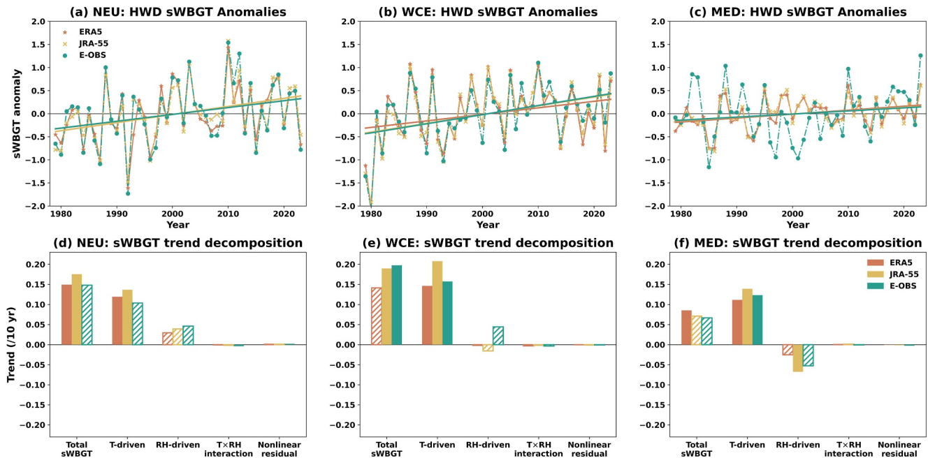
Figure 2. Regional sWBGT anomalies and trend decomposition during heatwave days, 1979–2023. (a–c) Annual sWBGT anomalies in NEU, WCE, and MED from ERA5, JRA-55, and E-OBS. (d–f) Trends in total sWBGT and its temperature-driven, RH-driven, T \times RH interaction, and nonlinear residual contributions. Solid and hatched bars indicate p < 0.05 and p \geq 0.05 , respectively, after lag-1 autocorrelation adjustment.
