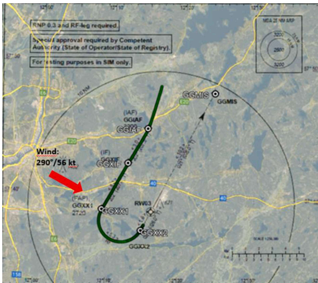
Fig. 14. Descending with a 3° from FAP/GGXX1, IAS 165 kt and CONF 2 with wind of 290°/56 kt.
