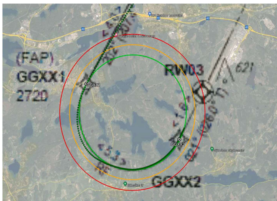
Fig. 16. Descending with a 3° from FAP/GGXX1, IAS 190 kt and CONF 2 with wind of 020°/56 kt; the radius of the RF leg (green circle), the outer limit of the RNP0.3 corridor (orange circle) and the outer limit of the protected area (the red circle). (For interpretation of the references to colour in this figure legend, the reader is referred to the Web version of this article.)
