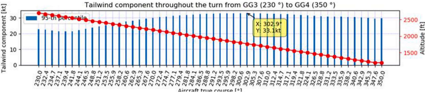
Fig. 5. The calculated TWC assuming a 3° descent angle throughout the fictitious turn from point GG3 to GG4 @ESGG.
