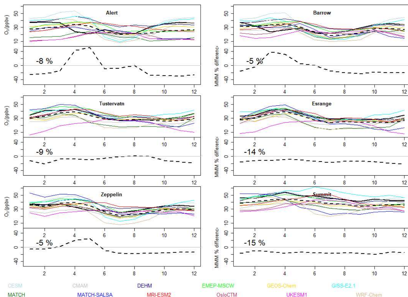
Figure 6. Arctic surface \text{O}_3 by month; seasonal cycle model comparisons. Top row: coastal high Arctic sites; middle row: sites near the Arctic Circle; bottom row: high-elevation sites. The solid black line is the observed \text{O}_3 monthly means, and the dashed black line is the multi-model median. Bottom row: sub-panels show the MMM percent difference [(\text{MMM} - \text{measurements})/\text{measurements} \times 100] . Note that model results are from the 2014–2015 mean. When available, the same years are used for the observations. However, Alert did not have data for 2014–2015, so its most recent years were used: 2010–2013. Summit had 2014 but only 1 month in 2015, so its 2013–2015 data were used.
