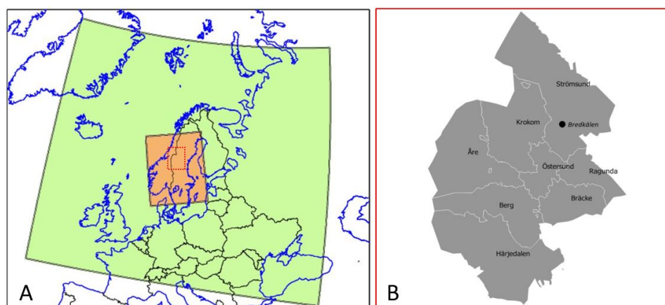
Figure 1. MACH domains covering northern Europe (panel A, green), at a 0.1^\circ \times 0.1^\circ resolution, and the inner domain covering Jämtland Härjedalen and surrounding areas (panel A, orange), at 4 \text{ km} \times 4 \text{ km} resolution. In panel (B) the Jämtland Härjedalen region municipalities are illustrated together with an approximate location of the EMEP station Bredkälen.
