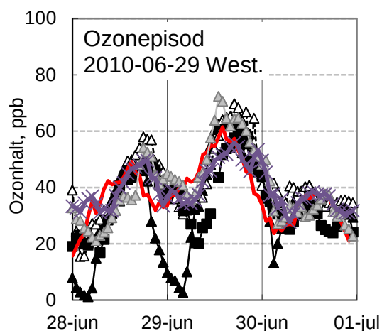
Figure 8.5: Hourly ozone concentrations measured with instruments in different parts of Sweden during the ozone episode of 2010-06-28 to 2010-06-30. For legends and locations, see Section 2.1 above. The red line included in all diagrams represents ozone concentrations at Vavihill, Skåne, for comparison.
