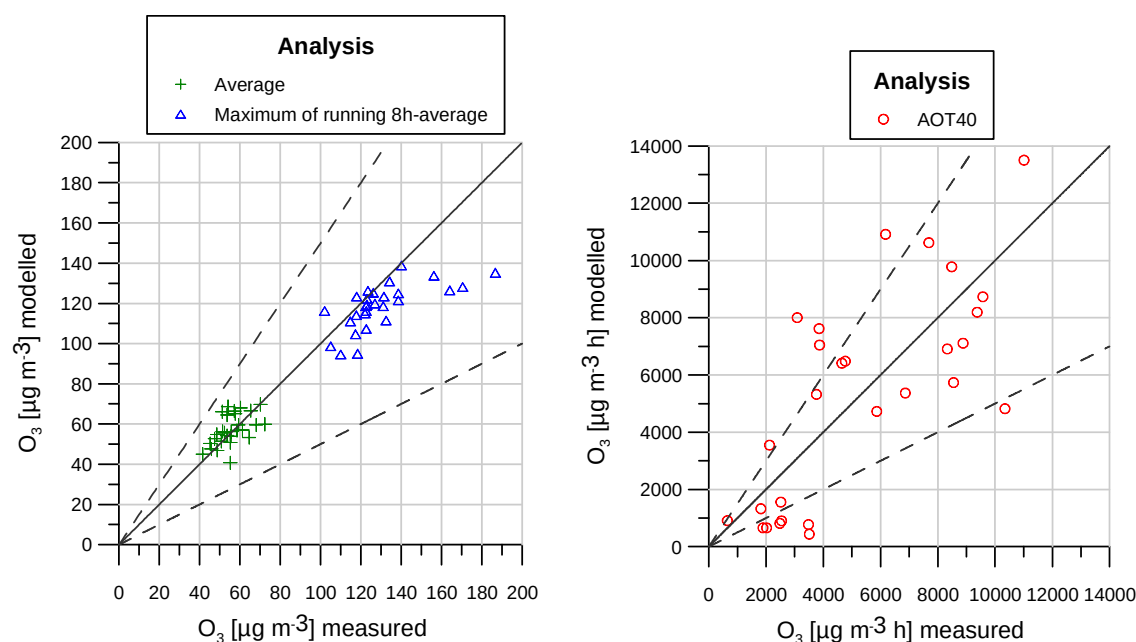
Figure 4.4: Scatterplots with summary of the comparison between measured and modelled concentration of ozone; annual mean values (green), annual maximum of running 8h-mean concentration (blue) and AOT40 (red). Each point is representing a station and a certain year. The continuous line represents 1:1 and dashed lines represent \pm 50\% . Numerical values are given in Table 4.1.
