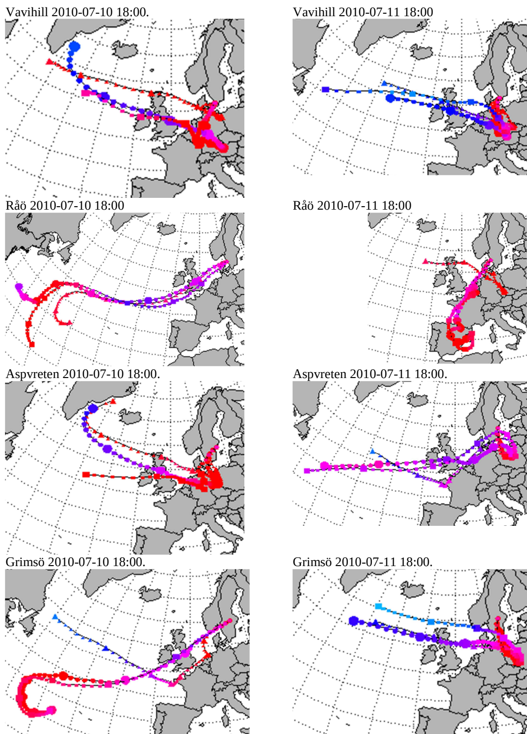
Figure 4.6: Trajectories for air masses arriving at Vavihill, Råö, Aspvreten and Grimsö during an ozone episode from 2010-07-10 to 2010-07-12, as estimated with the FLEXTRA model available at NILU. The time for arrival is indicated close to each diagram.
