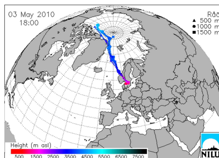
Aspvreten 2010-05-03.
