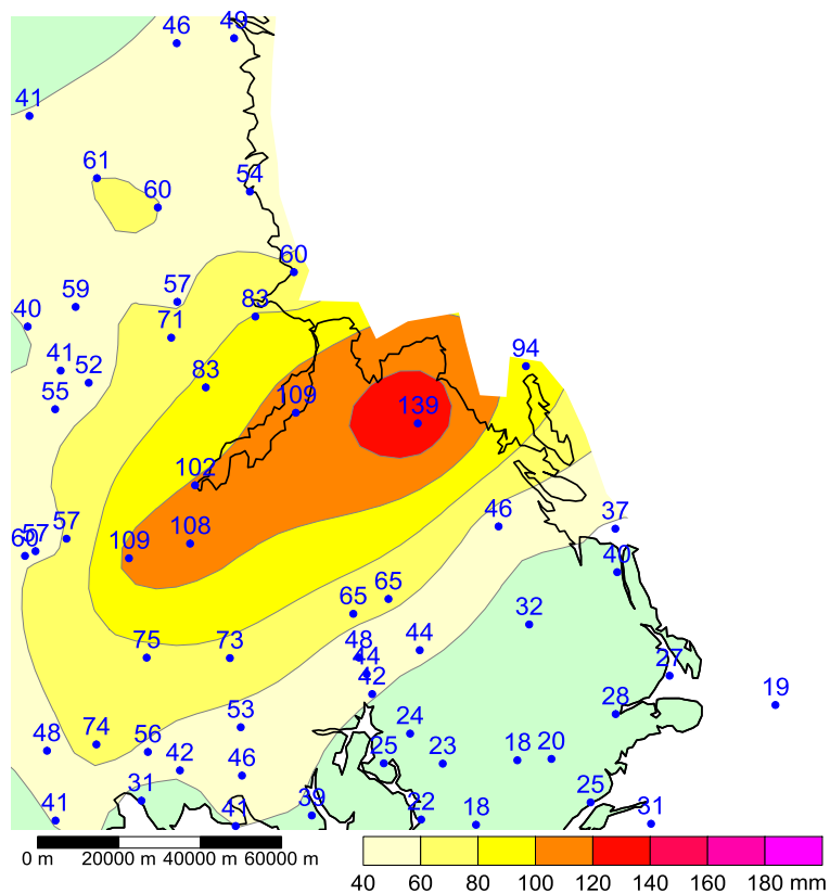
Figur 20. 1981-08-17 - 18 medel nbd 1000 km 2 : 120.0 mm area minst 90 mm: 4425 km 2
