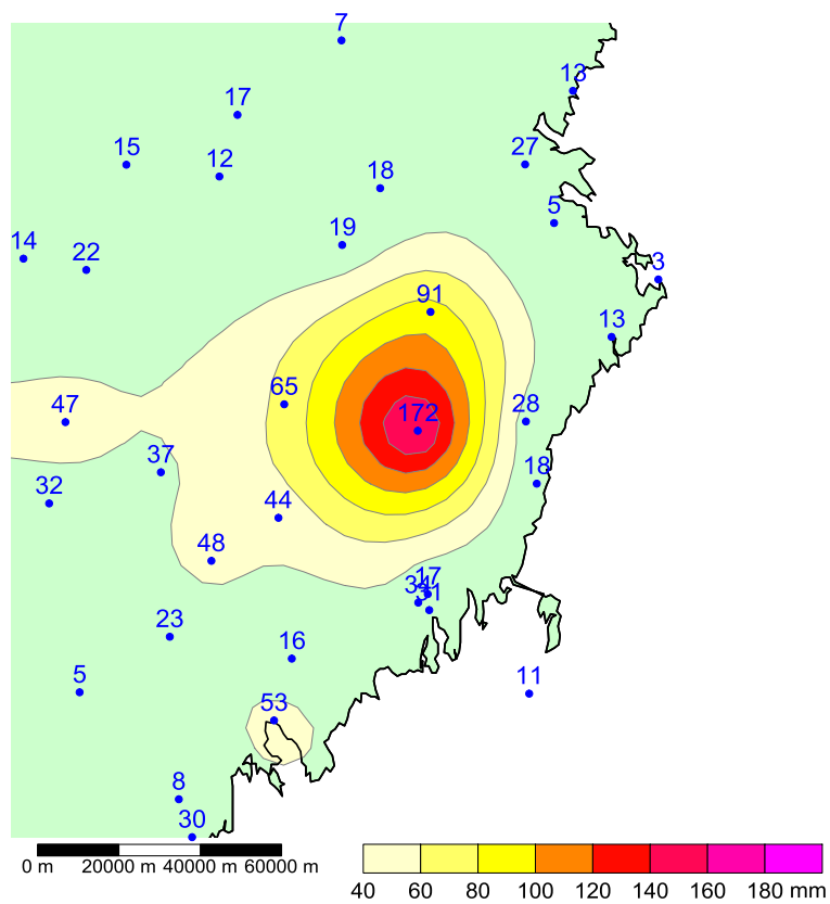
Figur 15. 1979-07-24 - 25 medel nbd 1000 km 2 : 122.1 mm area minst 90 mm: 1400 km 2
