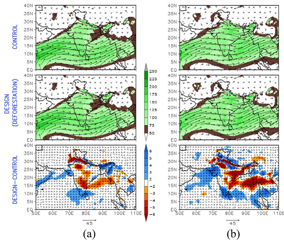
Fig. 6 The JJAS (2001–2010) composite mean and anomaly (design-control) of moisture transport at 850 hPa (kg/m/sec) for deforestation (a) RCM-DEF-UW (b) RCM-DEF-Holtslag, design experiments, respectively
