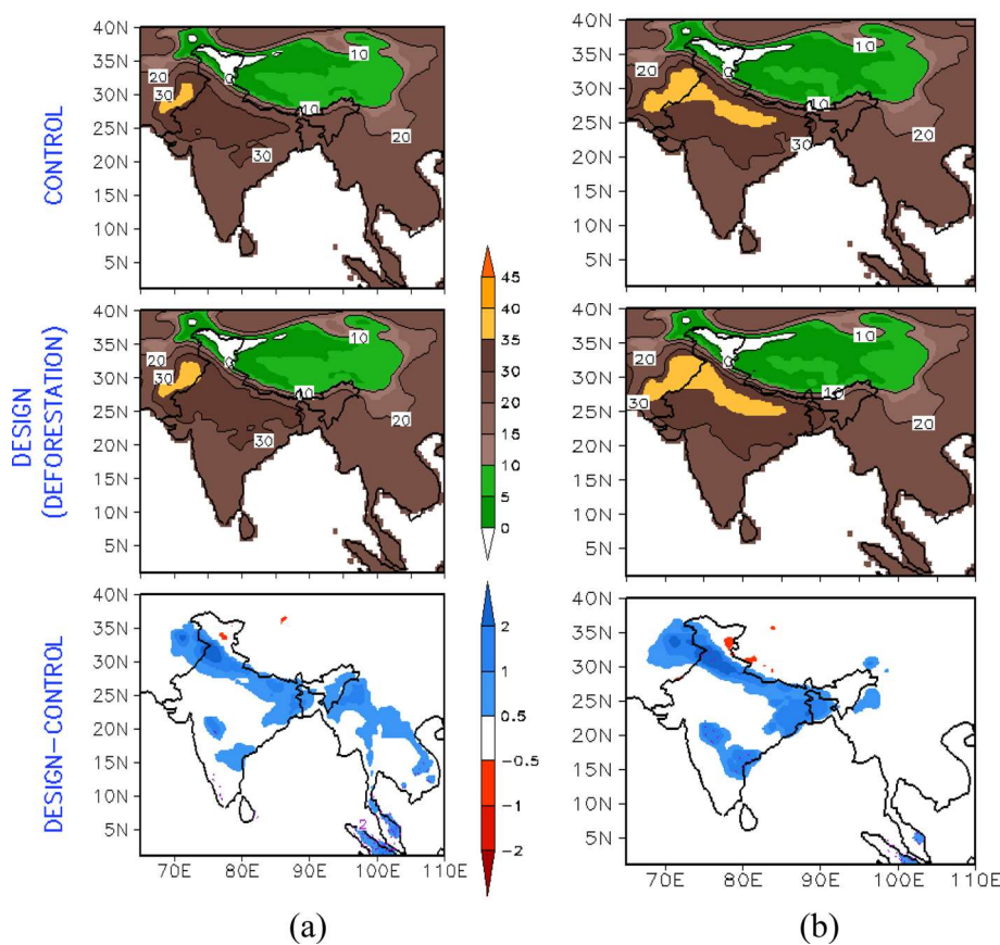
Fig. 9 The JJAS (2001–2010) composite mean and anomaly (design-control) ( p < 0.01 ) of near surface air temperature at 2 m ( ^{\circ}\text{C} ) for deforestation (a) RCM-DEF-UW (b) RCM-DEF-Holtslag, design experiments, respectively
