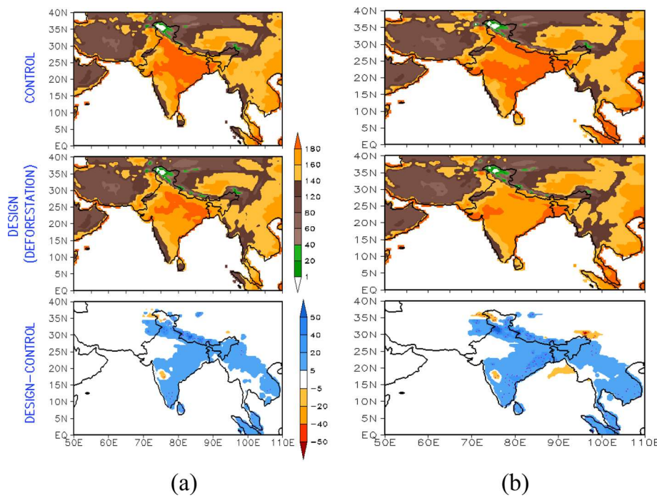
Fig. 14 The JJAS (2001–2010) composite mean and anomaly (design-control) of net upward longwave energy flux ( \text{Wm}^{-2} ) for deforestation ( a ) RCM-DEF-UW ( b ) RCM-DEF-Holtslag, design experiments, respectively
