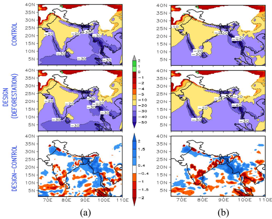
Fig. 7 The JJAS (2001–2010) composite mean and anomaly (design-control) of convergence of vertically integrated water vapor flux (mm/day) for deforestation (a) RCM-DEF-UW (b) RCM-DEF-Holtslag, design experiments, respectively
