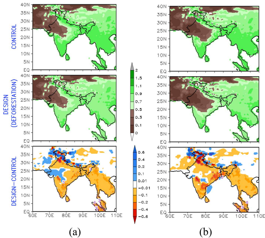
Fig. 13 The JJAS (2001–2010) composite mean and anomaly (design-control) of evaporative fraction for deforestation (a) RCM-DEF-UW (b) RCM-DEF-Holtslag, design experiments, respectively
