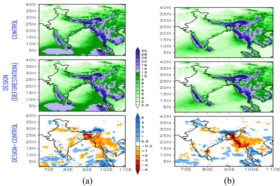
Fig. 2 The JJAS (2001–2010) composite precipitation (mm/day) and anomaly (design-control) for deforestation (a) RCM-DEF-UW (b) RCM-DEF-Holtzlag, design experiments, respectively. (The regions where there is decrease in precipitation is significant at 99% confidence level) [* (top) CONTROL exp, (middle) DESIGN exp; and (bottom) anomaly (design-control)]
