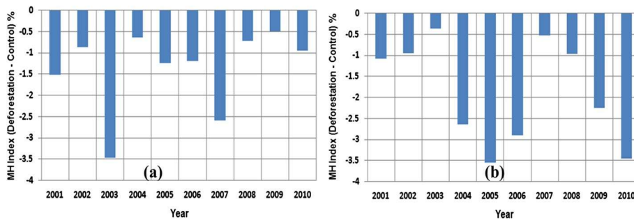
Fig. 8 Sensitivity of Monsoon Hadley (MH) index as calculated for deforestation (a) RCM-DEF-UW (b) RCM-DEF-Holtslag, design experiments, respectively
