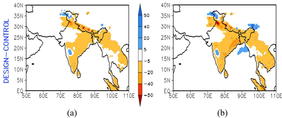
Fig. 16 The JJAS (2001–2010) composite mean and anomaly ( p < 0.01 ) of net radiation ( \text{W/m}^2 ) anomaly (design-control) (positive is downward) for deforestation (a) RCM-DEF-UW (b) RCM-DEF-Holtslag, design experiments, respectively
