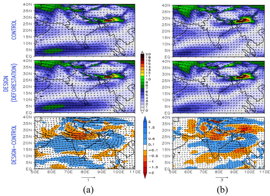
Fig. 4 The JJAS (2001–2010) composite wind (m/sec) anomaly (design-control) and change in direction at 500 hPa for deforestation (a) RCM-DEF-UW (b) RCM-DEF-Holtslag, design experiments, respectively
