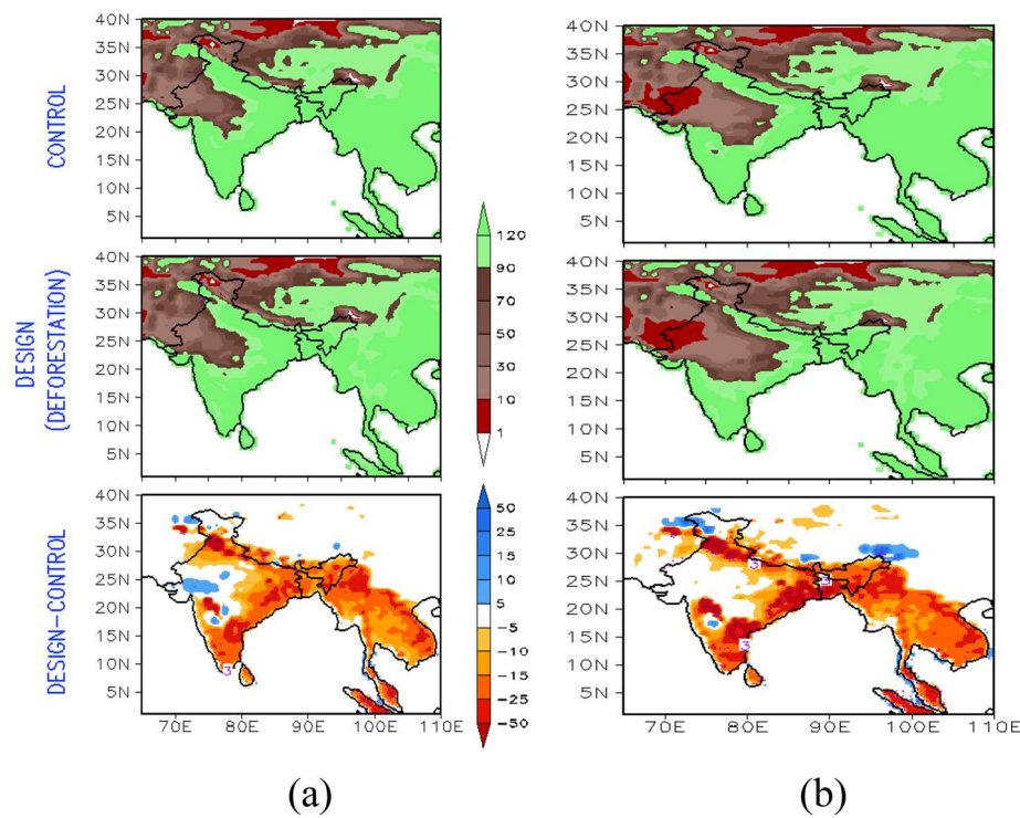
Fig. 12 The JJAS (2001–2010) composite mean and anomaly (design-control) of latent heat flux ( \text{Wm}^{-2} ) (a) RCM-DEF-UW (b) RCM-DEF-Holtslag, design experiments, respectively
