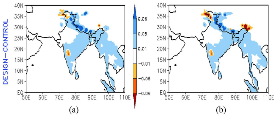
Fig. 15 The JJAS (2001–2010) composite mean and anomaly of albedo (design-control) for deforestation (a) RCM-DEF-UW (b) RCM-DEF-Holtslag, design experiments, respectively
