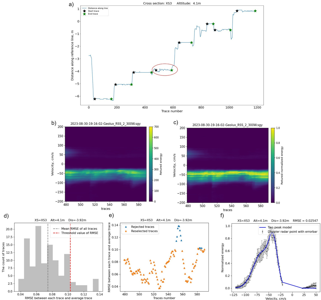
Figure 3. (a) Using XS3 as an example to show how to find the start and end trace in one waypoint. (b) And (c) show full waveform plots of the signal and the normalized signal energy based on the maximum of each trace at the same waypoint (indicated by the red circle in panel a), respectively. In (d), the Root Mean Squared Error (RMSE) between each trace and the Doppler normalized amplitude averaged over selected traces ( M_{data_{all}} ) at the waypoint (distance = -3.92 m). The vertical dashed red and gray lines indicate the selected max RMSE threshold and the mean RMSE value. (e) A comparison between reselected traces and rejected traces with RMSE values. In (f), black points indicate the normalized amplitude averaged over reselected traces ( M_{data_{new}} ). The error bars represent the standard deviation ( SD_{point} ) of comparing selected traces with M_{data_{new}} at the flow velocity value point by point. A Gaussian two peak model shown by the blue line was applied to fit M_{data_{new}} . Note that all results are calculated by using the normalized traces in panels (d)–(f).
