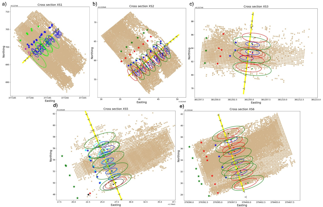
Figure 6. Shows the location of drone waypoints and footprints with different fly altitudes in SWEREF99 coordinates. In which, stars represent the locations of drone waypoints, and ellipses indicate the footprint area of Doppler radar equipped on the drone. Different colors denote the drone with different fly altitudes, details can be found in Figure 5. In addition, yellow lines represent the tagline of each cross-section, and the black circles are the locations of the tagline zero-point. Black left triangles along the tagline present the measuring positions by using OTT MF Pro. Finally, brown points in the area of coordinates are generated by using the PIV approach. Noted that cyan (2.1 m) and black (4.1 m) colors in panel (d) represent the measured waypoints and footprints before rain.
