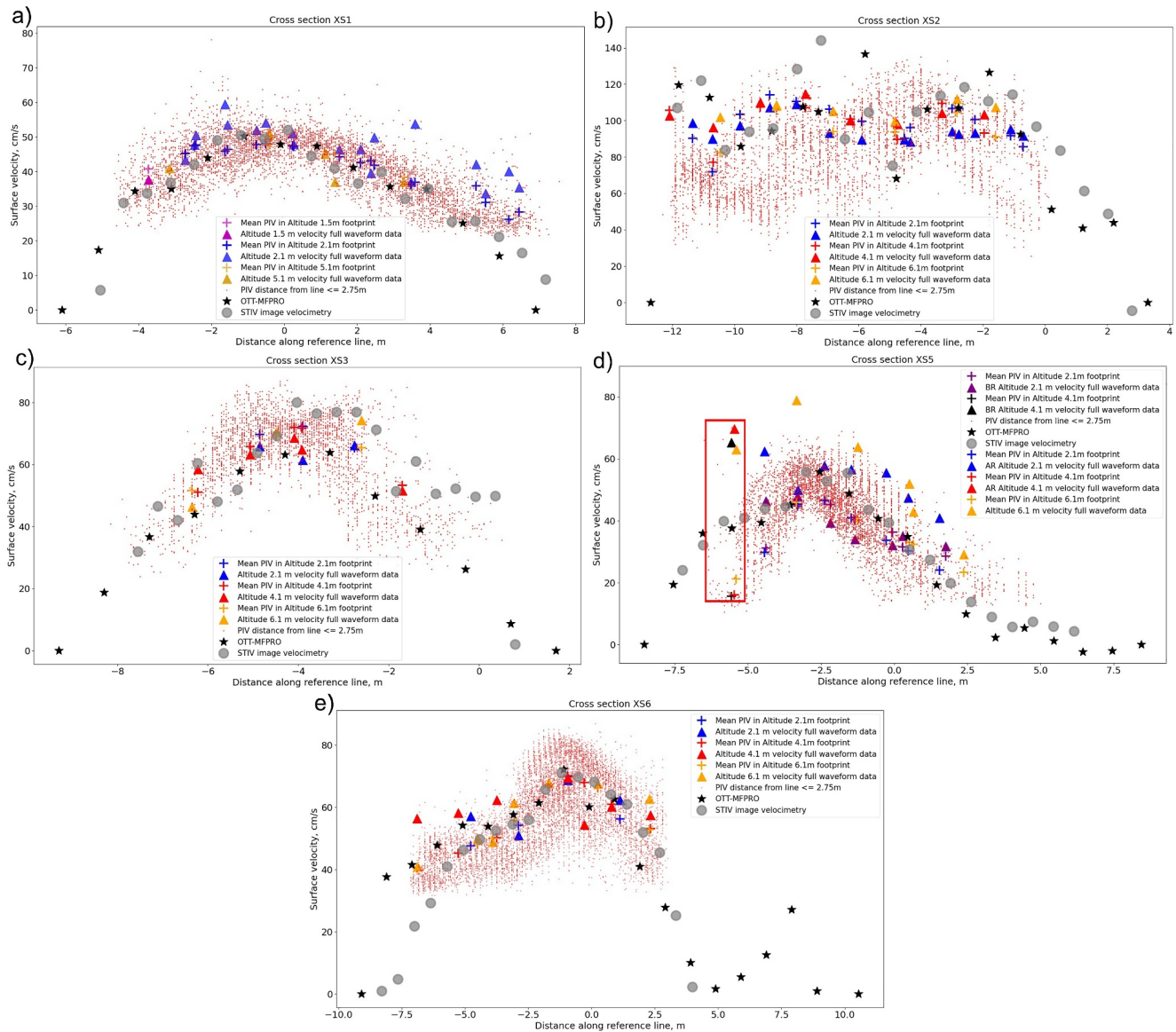
Figure 8. Comparisons of OTT MFPRO results (black stars), STIV image velocities (gray circles), velocities derived from Doppler radar full waveform data (triangle), PIV values by combining u and v component with distance from the tagline \leq 2.75 m (red points), and average PIV values in each elliptical footprint area (plus). Note that in panel (d), the red rectangle near -5.5 m shows a larger difference comparing Doppler radar results and PIV values, the main reason is the other drone's propwash effect during the PIV measuring process (see Figure 5d). A positive value means along the river flow direction.
