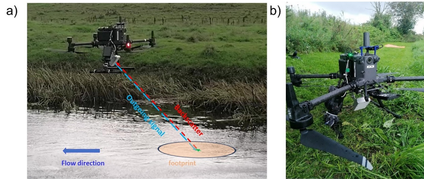
Figure 2. (a) Overview of UAS-borne Doppler radar located in one waypoint. Doppler radar always looks upstream, and considering the incidence angle ( 45^\circ ), the radar can receive the backscatter energy located in the ellipse area named footprint. (b) Shows the DJI Matrice 300 RTK carrying Geolux RSS-2-300W Doppler radar, the white square mounted below the main body of the drone.
