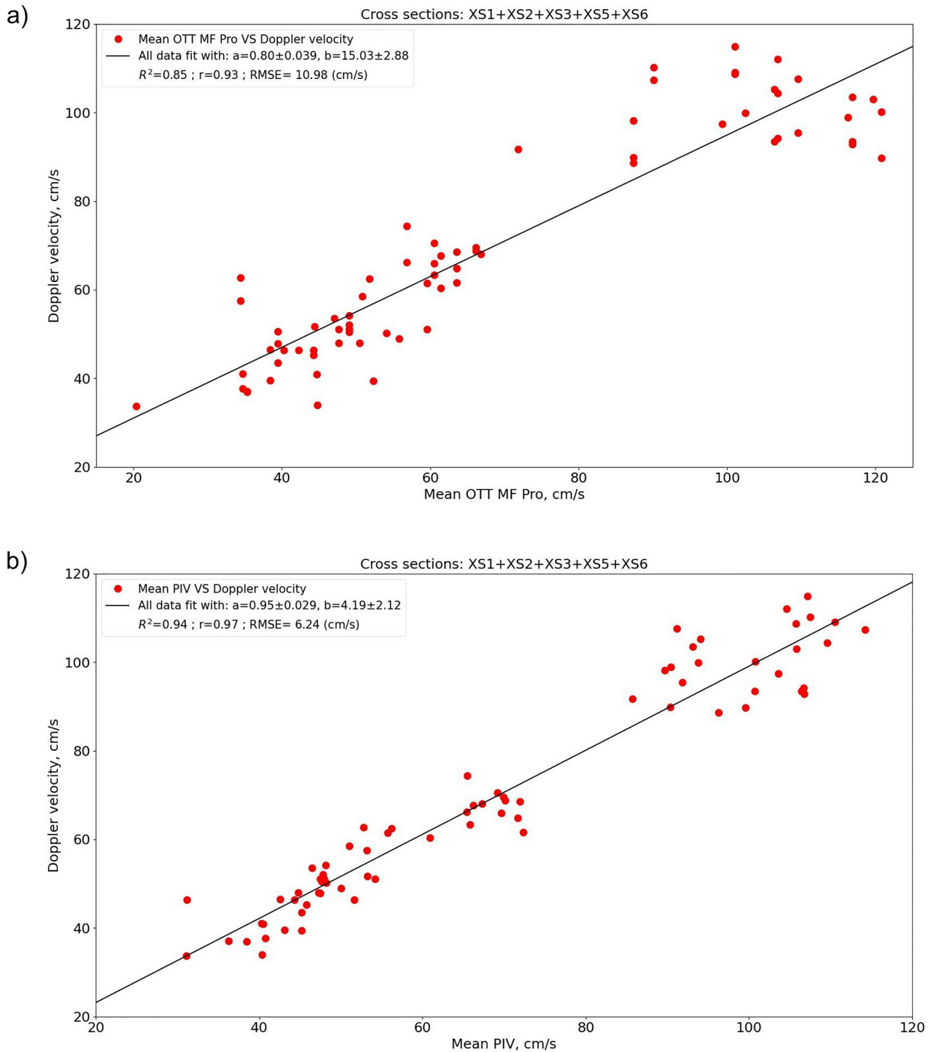
Figure B1. (a) And (b) show the correlations compared Doppler velocity with mean OTT MF Pro and mean PIV, respectively. For XS1, seven waypoints shown in Table 5 were discarded. For XS2, three waypoints close to -10.6 m were discarded. For XS3, all waypoints were kept and plotted in this figure. For XS5, we only retained four waypoints with both 2.1 m fly altitude and the measurement before the rain. For XS6, we discarded five waypoints with absolute errors larger than 20%. We also provided the coefficient of determination ( R^2 ), the Pearson correlation coefficient ( r ), and the RMSE value in legends of (a) and (b).
