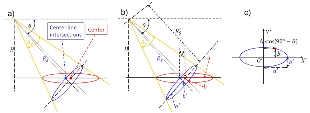
Figure A1. Visualizations of different steps to derive the footprint size of the drone with Doppler radar. In (a), the red ellipse is the ground projection, the blue is the beam size, and H is the altitude of the drone. The blue point is the center line intersection with the blue ellipse and the red point is the center of the projected footprint. \theta and \theta_r represent the tilt angle and the elevation angle, separately. In (b), the footprint ellipse consists of the major axis a and the minor axis b . In addition, the beam area is drawn by a blue ellipse with the major axis a' and the minor axis b' . And \Delta is the difference between the centerline intersection of the beam and the center of the footprint. R_s and R'_s represent the slant range from the drone to the river surface and the centerline intersection of the beam, separately. (c) Shows the beam area described with the X'Y' -coordinate system, the selected point marked as a red point with coordinate value X' = \Delta \cdot (\cos(90^\circ - \theta)) , Y' = b .
