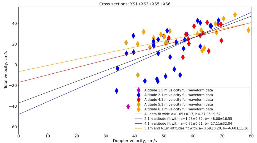
Figure 9. Shows the relation between Doppler velocities and total velocities, in which both were derived from Doppler radar full waveform data by using a Gaussian two peak model. Considering waypoints in XS1 with 5.1 m altitude, the average actual altitude is 5.84 m, therefore we combined 5.1 m altitude with 6.1 m together. From the results of different fly altitudes with 2.1 m, 4.1 m, and a combination of 5.1 and 6.1 m, we can obtain the drone-induced propwash velocities become smaller as flight altitude increases. Note that, a positive value means along the river flow, the propwash velocity caused by the drone is always against the river flow. In addition, to fit these straight lines in this figure, we discarded some waypoints, which were not fitted well with PIV results or were too small for total velocities.
