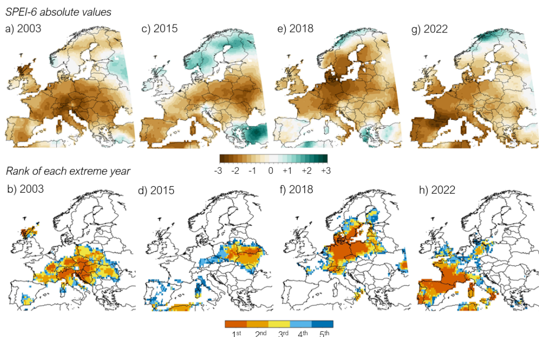
Figure 3. Comparison of the SPEI6 for September of the main Europe-wide droughts since 2000: namely, 2003, 2015, 2018, and 2022 (a, c, e, g) and their associated ranking (b, d, f, h). The period analysed is 1950–2022. A rank of one signifies that SPEI6 September for a given year (i.e. 2003, 2015, 2018 or 2022) is record-breaking, i.e. the lowest value during the analysed period.
