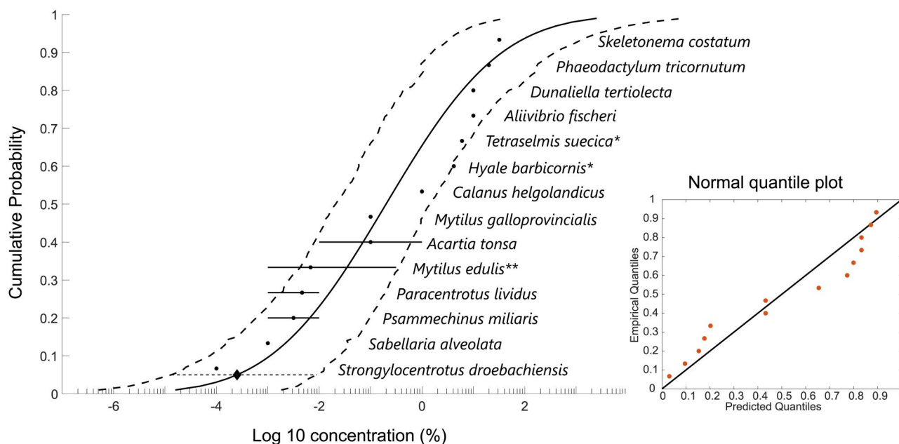
Figure 1. Species sensitivity distribution curve of open loop scrubber exposure from ships and laboratory scrubber based on chronic no observed effect concentrations. *Acute lethal concentration of 50% of the tested species converted to chronic equivalent by multiplying by 1/10. **Chronic effect concentration of 50% of the tested species converted by multiplying by 1/3 (follow the procedure of Posthuma et al., 2019). Hazardous concentration for 5% = 0.0003% (lower level = 0.00001%, upper level = 0.009%). Solid line, log-normal fitted distribution; dashed lines, lower and upper 95% confidence limits.
