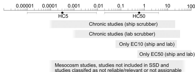
Figure 2. The data range of ecotoxicological effect concentrations of open loop scrubber exposure, including laboratory scrubbers. The range of chronic studies includes the no observed effect concentration, the lowest observed effect concentration (if the lowest tested concentration yields an effect), and the effect concentration of 10% of the tested species (EC10). The acute range includes the effect concentration of 50% of the tested species (EC50). Mesocosm studies are based on no observed effect concentrations, and the range of all effect concentrations from the excluded studies represents that of all available reported effect concentrations. HC5 = hazardous concentration for 5%; HC50 = hazardous concentration for 50%.
