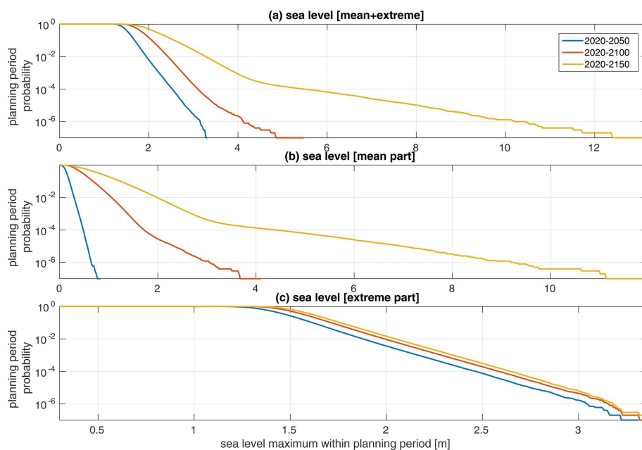
Figure 3. Planning period probability of sea level maximum for three different lengths of the planning period. Panel (a) shows the joint sea level maximum, (b) the maximum mean sea level and (c) the maximum extreme sea level. The figure is derived using the mean sea level projection probabilities given in Table 1.
