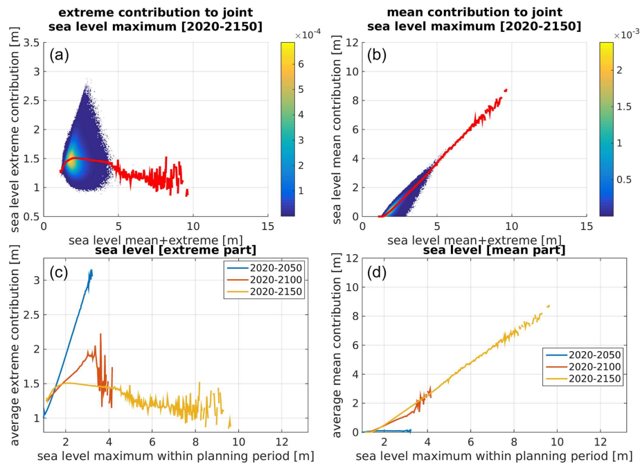
Figure 8. Mean sea level and extreme sea level contributions to joint sea level maximum. Upper panels (a, b) show relative density [unitless] of the extreme and mean sea level contributions to the joint sea levels. The lower panels (c, d) show average extreme and mean sea level contributions for different lengths of the planning period. Similarly, the red lines in panels (a) and (b) show the average extreme and mean sea level contributions for the 2020–2150 planning period.
