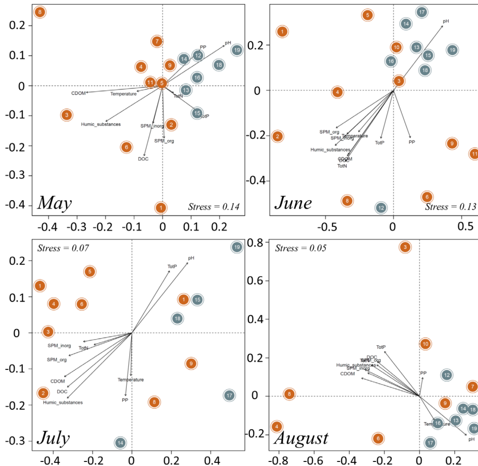
Fig 2. Non-metric multi-dimensional scaling (nMDS) analysis of variations in the bacterial community structure at different stations in the estuary during May, June, July and August. Numbers within circles denote station number. The analysis is based on Bray–Curtis dissimilarity values applied to relative abundances of OTUs. Colours denote inner (light brown) and outer estuary (light blue). Arrows denote the vector averages of each environmental parameter fitted in the ordination model defined by OTUs relative abundance data. The significance of each vector was assessed with a goodness-of fit statistics ( r^2 ) using 1000 permutations. [Color figure can be viewed at wileyonlinelibrary.com ]
