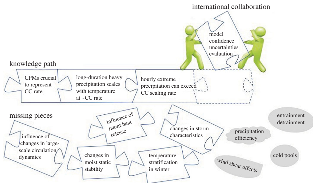
Figure 2. Knowledge path on relationship between precipitation extremes and global warming: consensus and missing pieces. Additional studies are required to dissipate uncertainties linked to the influence of large-scale circulation dynamics, latent heat release and moist static stability, changes in storm characteristics and temperature stratification. International collaboration is needed to increase model confidence, to evaluate uncertainties and to advance scientific knowledge on poorly understood phenomena like cold pools, wind shear and precipitation efficiency. (Online version in colour.)
