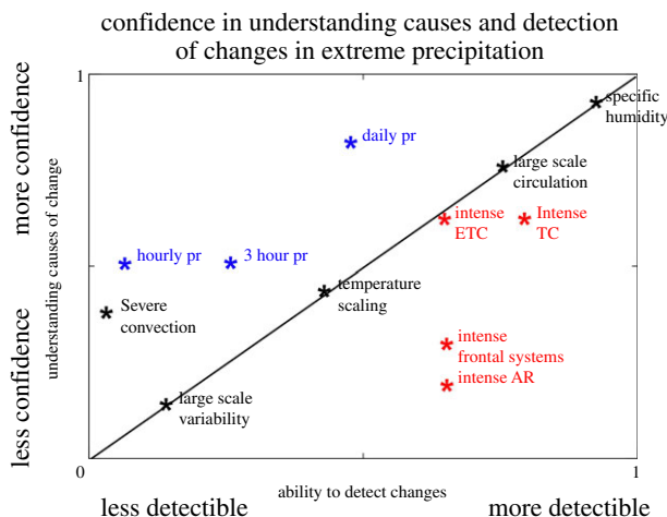
Figure 3. Confidence in understanding causes and detection of changes in extreme precipitation. (Online version in colour.)
