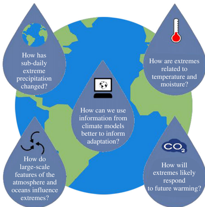
Figure 1. The INTENSE project's key questions. (Online version in colour.)
